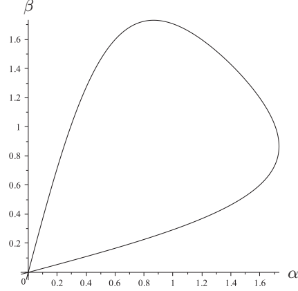
Figure 3: The curve (18) in \mathbb{R}_+^2 for z = 1/4 .
