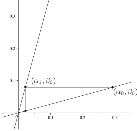
Figure 4: The curve (18) near 0 for z = 1/4 , and the construction of the products: the \alpha_k and \beta_k are given by the intersections of the curve (18) with the broken line.
