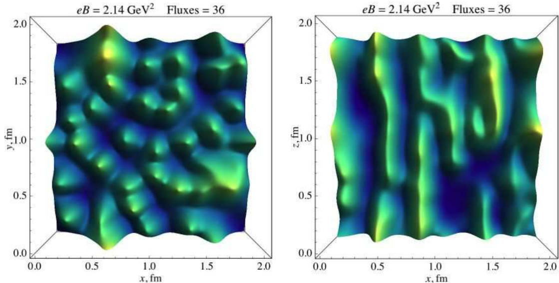
Fig. 17. A on-top view of the typical behavior of the Abelian energy density (142) in (left) the (x, y) plane and (right) the (x, z) plane for magnetic field eB = 2.14 \text{ GeV}^2 . The energy density was interpolated for a better visualization. In the left plot the magnetic field is perpendicular to the page while in the right plot the magnetic field is directed vertically (from Ref. [91]).
