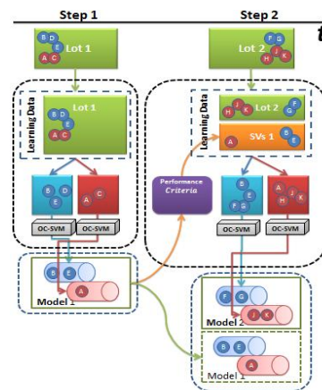
Figure 1. Schema of mOC-iSVM.EP
