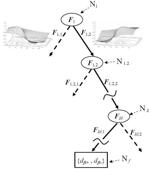
Fig. 5. The structure of the fuzzy decision trees used at the discriminant level.
