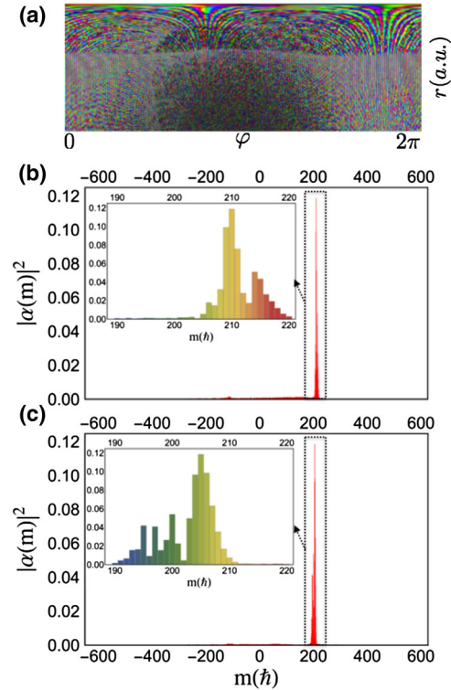
FIG. 3 (color online). (a) Calculated phase distribution of the electron wave function around the first order of diffraction. This is calculated by Fourier transforming the experimentally determined transfer function of the hologram from a measured map of the hologram thickness [see Fig. 1(c)]. The phase distribution is shown in polar coordinates, where the phase value is represented in a hue color. The OAM spectrum of the generated beam at the first order of diffraction from the hologram with and without the central dead region are shown in (b) and (c), respectively. This is measured by performing a one-dimensional Fourier transform of the azimuth coordinate. Because of imperfections at the origin and low spatial frequency for the case of (b), the beam is not pure and the value of OAM is delocalized centered around an OAM of (210.95 \pm 0.030)\hbar , while for the hologram with the excluded central dead region (c) the OAM spectrum central peak is about (202.75 \pm 0.032)\hbar . Indeed, the OAM spectrum, for both cases, moves to higher values mainly due to a small contribution from the second order of diffraction which carries an OAM of 400\hbar [see Fig. 2(b)]. Nevertheless, the hologram with the excluded central dead region (c) gives much better results.
