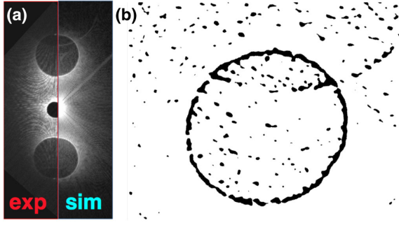
FIG. 2 (color online). (a) Experimentally (exp) observed and simulated (sim) Fraunhofer diffraction of a conventional EB from the CGH of Fig. 1(b). The upper and lower bright doughnuts are the \pm 1 orders of diffraction. In order to increase the visibility of the first order of diffraction, the central beam is blocked by a beam stop. The hologram is symmetric, and thus both first orders of diffraction possess the same OAM value, nonetheless having an opposite sign. The distribution of the electrons that possess a phase singularity at the upper side (a) is calculated and shown in (b). The singularity tends to concentrate in a ring at the periphery of the dark region. This is achieved by measuring phase variation about an infinitesimal region close to each pixel at the upper diffraction area. As can be seen, the residual of the second order of diffraction with an OAM value of 400\hbar (upper doughnut) is partially superimposed with the beam of first order. This lies in the fact that the diffraction angle of the electrons leaving the hologram is smaller than the divergence angle of the EB. Similar results are achieved for the hologram that its central region, shown in Fig. 1, is blocked.
