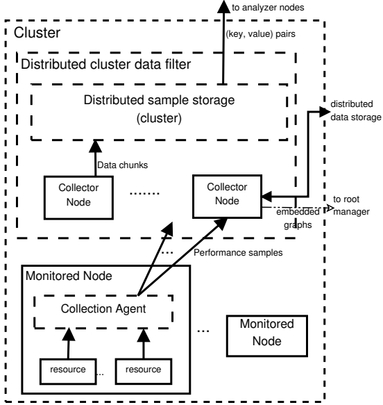
Figure 2: Cluster architecture
