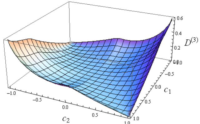
Fig. 2 Genuine Tripartite Quantum Discord for a_1 = 0 (notice that the maximum value of z axis is set to 0.6 and not to 1.0 in order to make the graph more readable).
