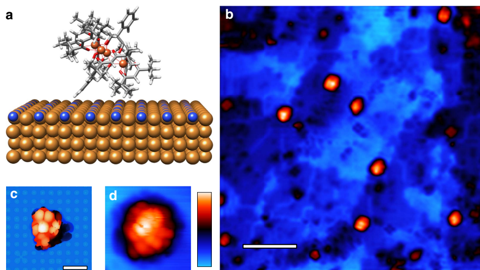
Figure 1 | \text{Fe}_4 molecule adsorbed on the \text{Cu}_2\text{N} surface. (a) [\text{Fe}_4(\text{L})_2(\text{dpm})_6] resting on the \text{Cu}_2\text{N} surface. Adsorption geometry and molecular structure are computed by density function theory (DFT). The molecule's axis defined by the tripodal ligands is at a 33^\circ angle from the surface normal. Atoms are Fe (orange), O (red), C (grey), H (white), Cu (brown) and N (blue). (b) Overview scanning tunnelling microscope (STM) image of the \text{Cu}_2\text{N} surface after deposition of molecules (scale bar, 8 nm). A number of \text{Fe}_4 molecules are visible as the tallest objects in orange. This image was filtered to remove noise using WSxM software 23 . (c) Calculated top view image of relaxed \text{Fe}_4 on \text{Cu}_2\text{N} showing the spatial distribution of the density of states integrated between 0 and +3 eV in energy. (d) STM image of an \text{Fe}_4 molecule. It appears as a spheroid of \sim 2 nm diameter with a multi-lobed substructure consistent with the calculated image in (c). The colour scale indicates the topographical height ranging between 0 and 1 nm in (b,d), which were acquired at a tunnel current set-point of 3 pA and bias voltage of 2.3 V. The 1-nm lateral scale bar inset in (c) also applies to (d).
