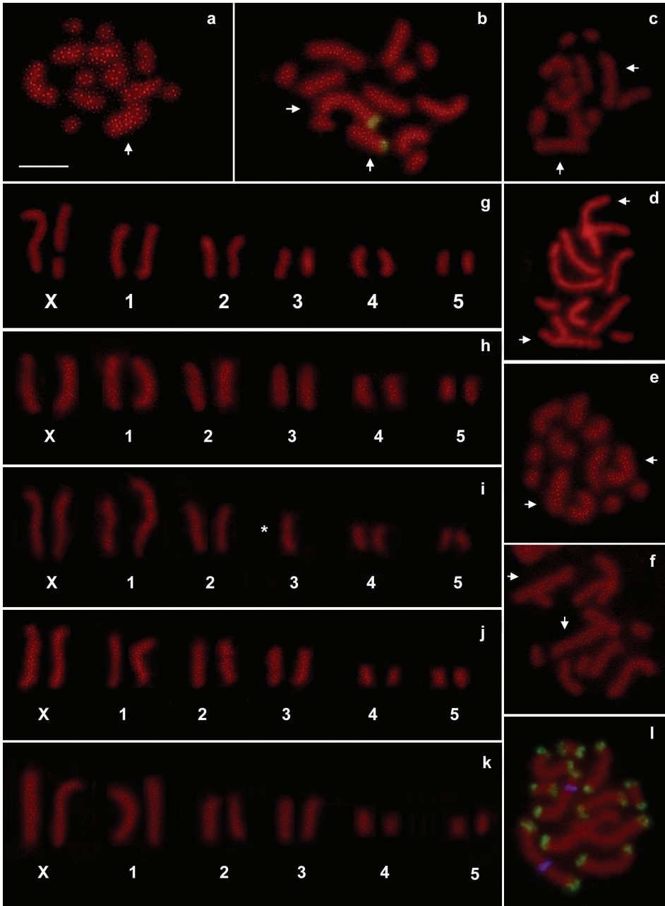
Figure 2. Chromosomal plates (a, c–f) and karyotypes (g–k) obtained from specimens belonging to clones Re1 (a, g, e) Re2a (c, h), Re2b (d, i), Re3 (e, j) and Re4 (f, k). Fluorescent in situ hybridization with the 28S probe (in green) (b) revealed that the fragmentation at the X chromosome in clone Re1 occurred at the telomere opposite to the NOR (b). Simultaneous in situ hybridization with the histone (in blue) and subtelomeric DNA probes (in green) in clone Re2b (i) revealed that the A1–A3 translocation involved the autosome 1 telomere close to the histone cluster. Arrows indicate X chromosomes. Asterisks indicate rearranged autosomes. Bar = 10 mm.
