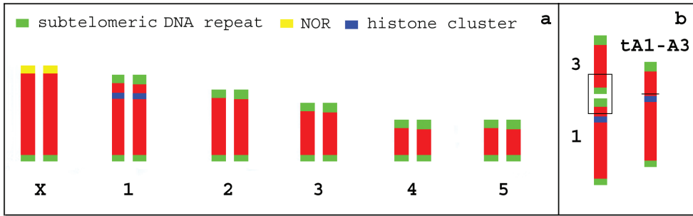
Figure 4. According to previous studies (Spence et al. 1998, Mandrioli and Manicardi 2012), the standard karyotype of M. persicae females consists of five couples of autosomes and two X chromosomes, whose rearrangements can be studied using different chromosomal markers (the subtelomeric DNA repeat, the NOR regions, and the histone cluster) (a). The analysis of karyotypes of clone Mo3, Mo4 and Re1 indicated that the observed A1-A3 translocation involved the A1 telomere near to the histone cluster and resulted in the loss of both the subtelomeric and the telomeric sequences (b).
