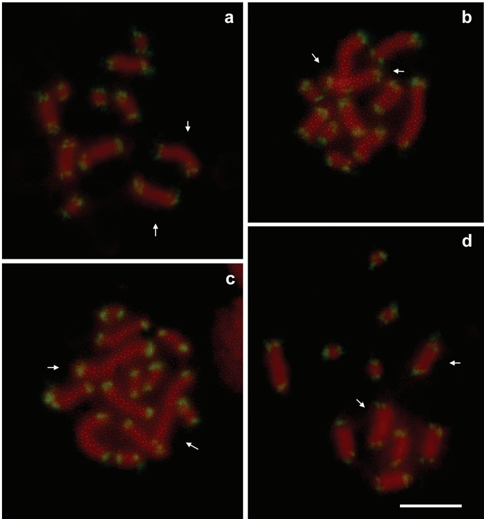
Figure 3. FISH with the telomeric (TTAGG)_n probe showed evident telomeric repeats at each chromosome in clones Mo3 (a), Mo4 (b), Re1 (c) and Re2b (d). No interstitial telomeric signals were present in clones Mo3 (a), Mo4 (b) and Re2b (d) possessing a chromosome derived from an autosome A1–A3 fusion. All telomeres resulted labelled by the (TTAGG)_n telomeric probe in clone Re1 including the X chromosome involved in the fission suggesting that a de novo telomere synthesis occurred in this clone (c). Arrows indicate X chromosomes. Bar = 10 \mu m.
