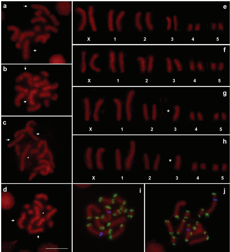
Figure 1. Chromosomal plates ( a–d ) and karyotypes ( e–h ) obtained from specimens belonging to clones Mo1 ( a, e ) e Mo2 ( b, f ), Mo3 ( c, g ) and Mo4 ( d, h ). Simultaneous in situ hybridization with the histone (in blue) and subtelomeric DNA probes (in green) ( i–j ) revealed in both clones Mo3 ( i ) and Mo4 ( j ) that the A1–A3 translocation involved the autosome 1 telomere close to the histone probe. Arrows indicate X chromosomes; asterisks indicate rearranged autosomes. Bar = 10 mm.
