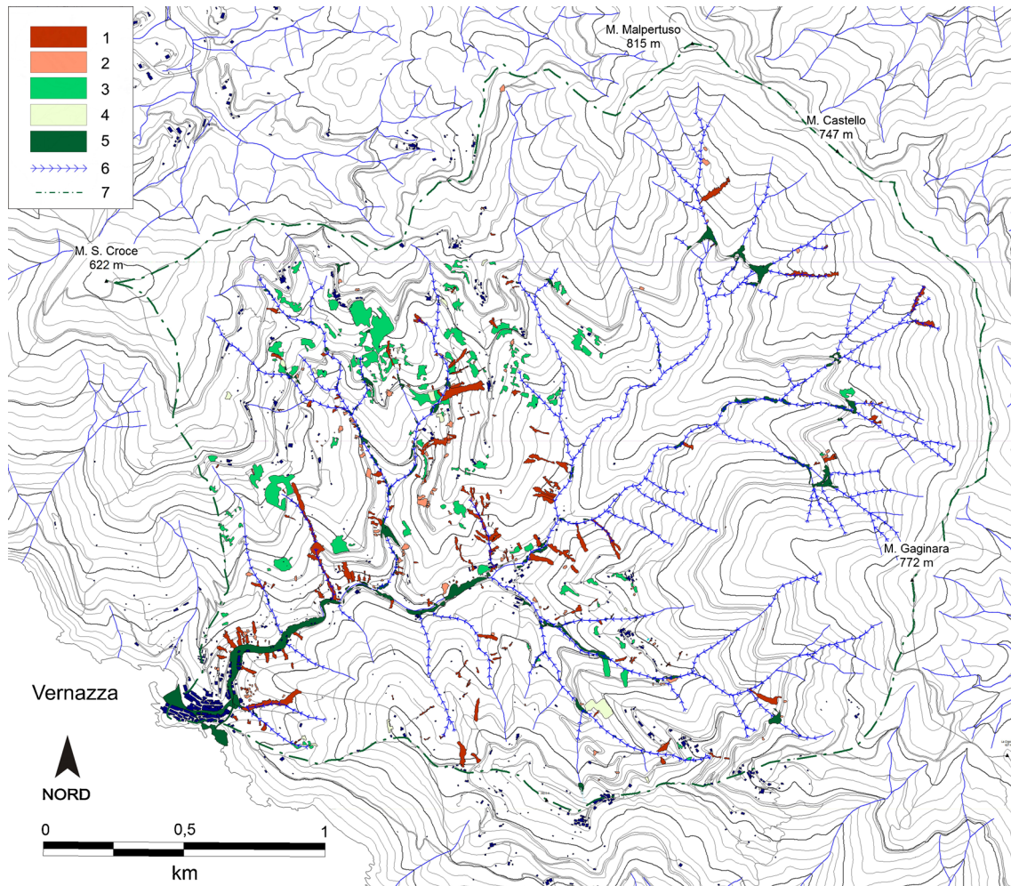
Fig. 5 Map of shallow landslides and erosional processes induced by rainfall on October 25, 2011 (after Cevasco et al. 2013a). Legend: 1 flow; 2 slide; 3 widespread outwash; 4 rill/gully erosion; 5 debris flood deposit; 6 downcutting talweg; 7 watershed boundary
