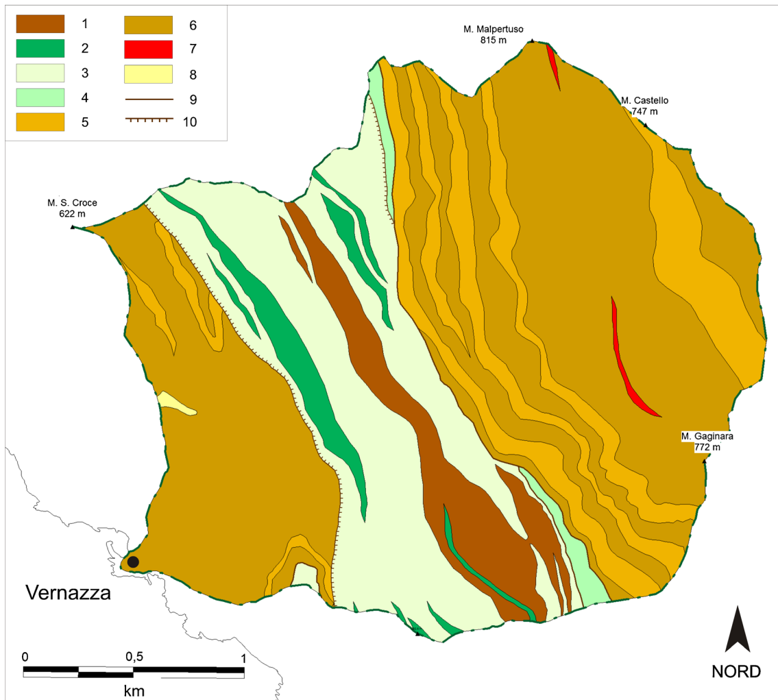
Fig. 2 Geological map of the Vernazza catchment (after Regione Liguria 2006a, modified). Legend: 1 Ponte Bratica Sandstones; 2 Groppo del Vescovo Limestones; 3 Canetolo Shales and Limestones; 4 T. Pignone Marls; 5 Macigno Fm.; 6 Macigno Fm.—fine-grained sandstone lithofacies; 7 Macigno Fm.—pelitic and silty lithofacies; 8 Macigno Fm.—silty-marly lithofacies; 9 reverse faults and overthrusts; 10 direct faults
