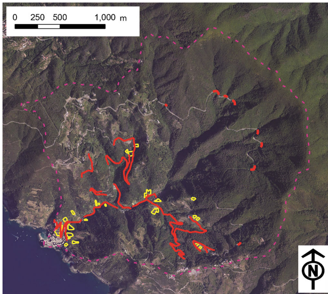
Fig. 11 Stretches of roads selected to be protected (in red) and location of hillslopes chosen to apply structural measures to avoid damages on buildings caused by landslides (in yellow). Vernazza catchment is indicated with a dashed purple line (orthoimage source: Bing Maps)
