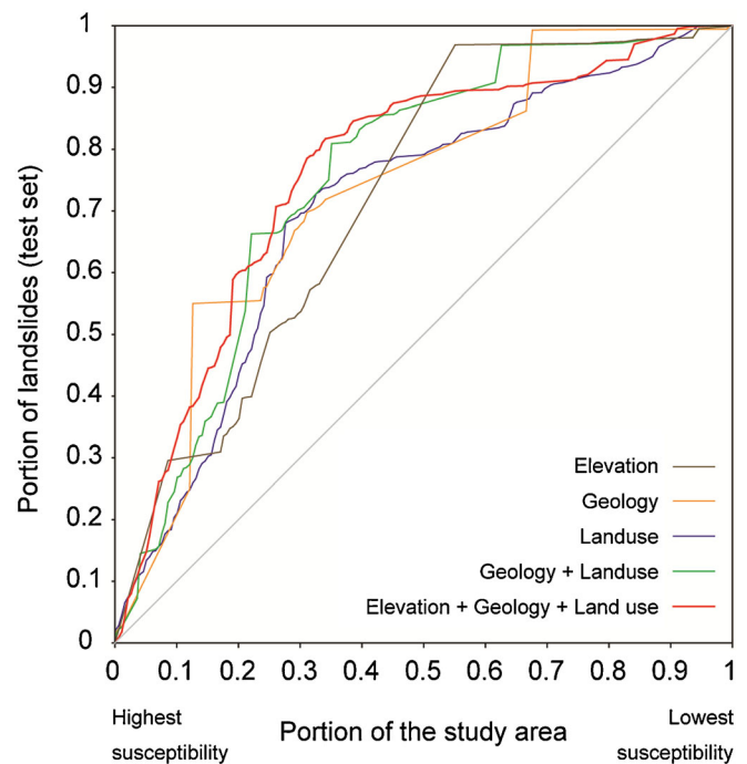
Fig. 7 Prediction rate curves (PRCs) for the more significant models. PRCs are cumulative frequency curves that indicate the proportion of landslides in the test set that occurs within a certain proportion of the area with the highest susceptibility (Chung et al. 1995). The larger the area between the PRC and the diagonal (grey line), the greater the prediction capability of the model
