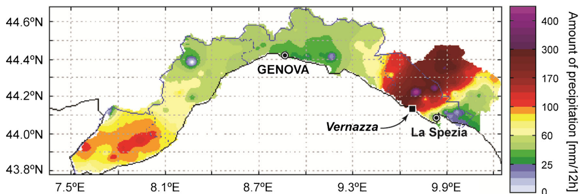
Fig. 3 Twelve-hour cumulative rainfall estimated at 1800 UTC in Liguria region during the event of October 25, 2011 (after ARPAL-CFMI-PC 2012, modified)
