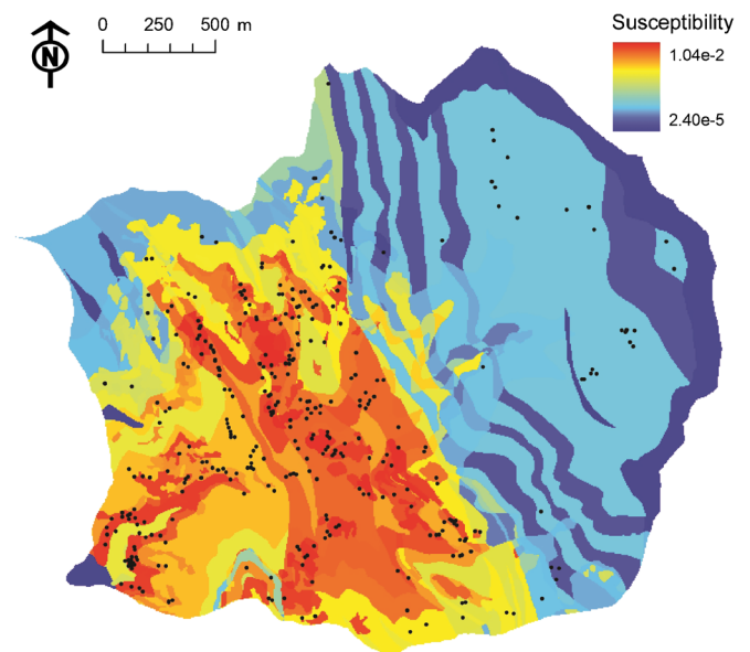
Fig. 9 Susceptibility map produced for the Vernazza catchment. The landslide source areas used for producing the map have been indicated with black points. Susceptibility values indicate the spatial probability of the pixels to be a landslide source area for a landslide event equal to the one that occurred on October 25, 2011
