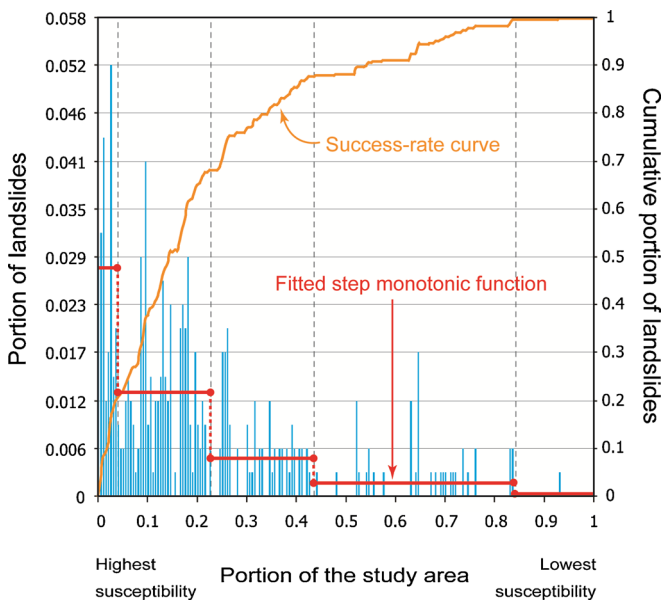
Fig. 8 Histogram plot (blue columns) representing the proportion of landslides in each susceptibility class from the highest to the lowest susceptibility classes. Red line indicates the estimated empirical areal frequency of landslides based on a fitted step (or discontinuous) decreasing monotonic function. The limits of the stretches of this monotonic function were defined according to the slope changes observed in the success rate curve (SRC) (orange line). The SRC is a cumulative frequency curve that indicates the proportion of the landslide population that occurs within a certain proportion of the area with the highest susceptibility (Chung and Fabbri 1999). The use of a monotonic function involves some loss in spatial resolution because this transformation reduces the number of susceptibility classes but it is necessary to overcome the land use change simulations. Similar approaches that use monotonic functions have been applied to produce probabilistic models by Fabbri et al. (2004), Zêzere et al. (2004), Chung (2006) and Galve et al. (2011)
