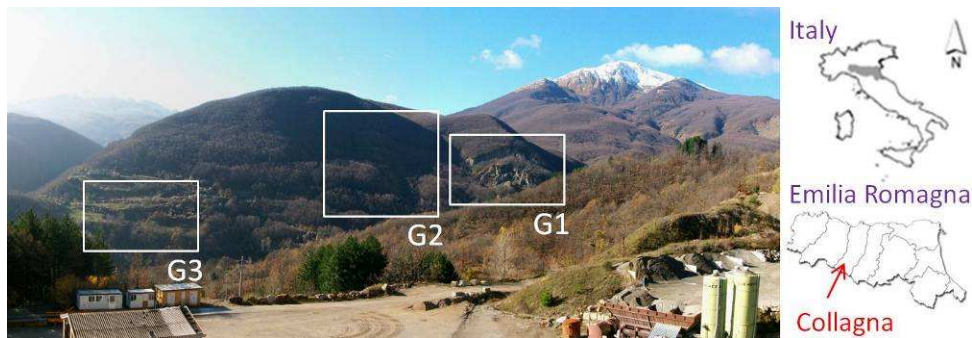
Figure 1: Photograph and geographical location of the Col Piagneto landslide. White rectangles evidence the three sectors of the landslide.
