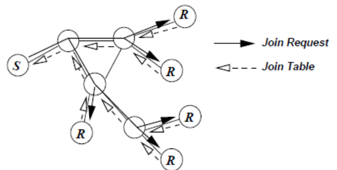
Fig.1: On-Demand Procedure for Membership Setup and Maintenance.
