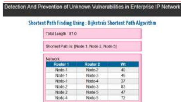
Figure 4. Shortest path
