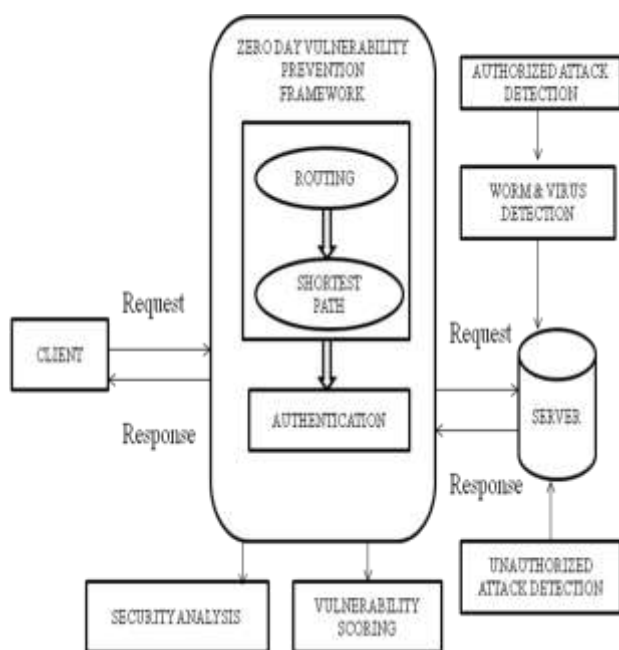
Figure 3. System Architecture
