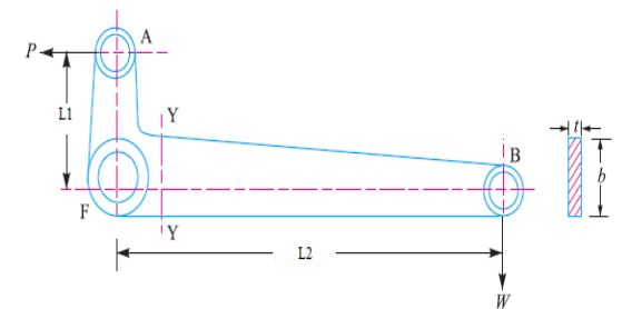
Figure1- Bell Crank Lever
