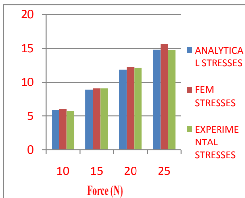
Figure26 - Comparison of Maximum Stresses Analysis by Analytical, FEM and Photoelasticity of Bell Crank Lever.
