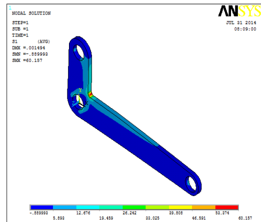
Figure11- 1 st Principal Stress Optimization for Volume of Bell Crank Lever.
