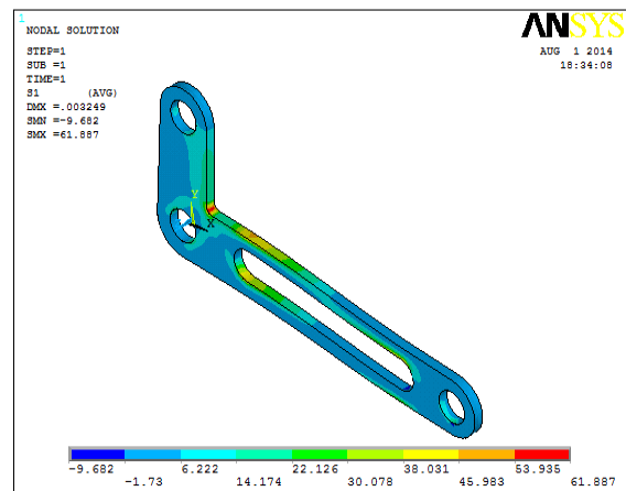
Fig. 15- 1 st Principal Stresses of Bell Crank Lever Increasing 3 Holes.
