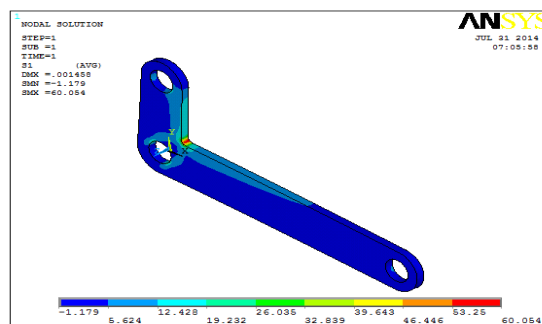
Figure5.- 1 st Principal Stress of Bell Crank Lever with Fillet Radius 4 mm.
