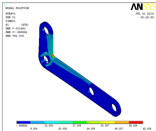
1 st Principal Stresses of Bell Crank Lever Increasing 1 Hole.
