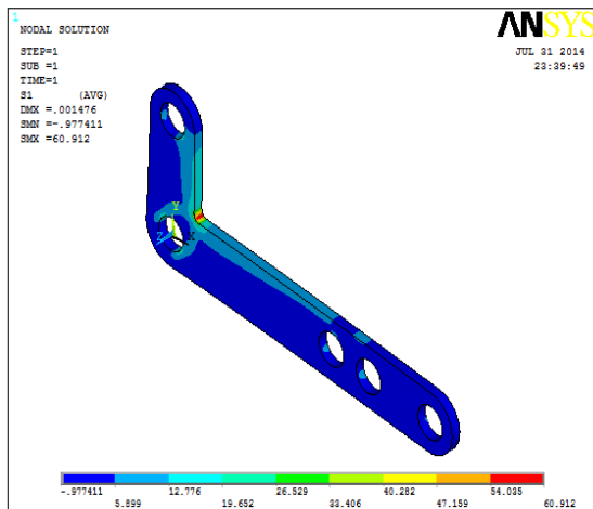
- 1 st Principal Stresses of Bell Crank Lever Increasing 2 Holes.
