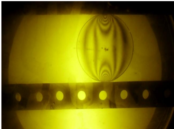
Figure.17. Isochromatic fringe pattern developed in circular disc under compression
