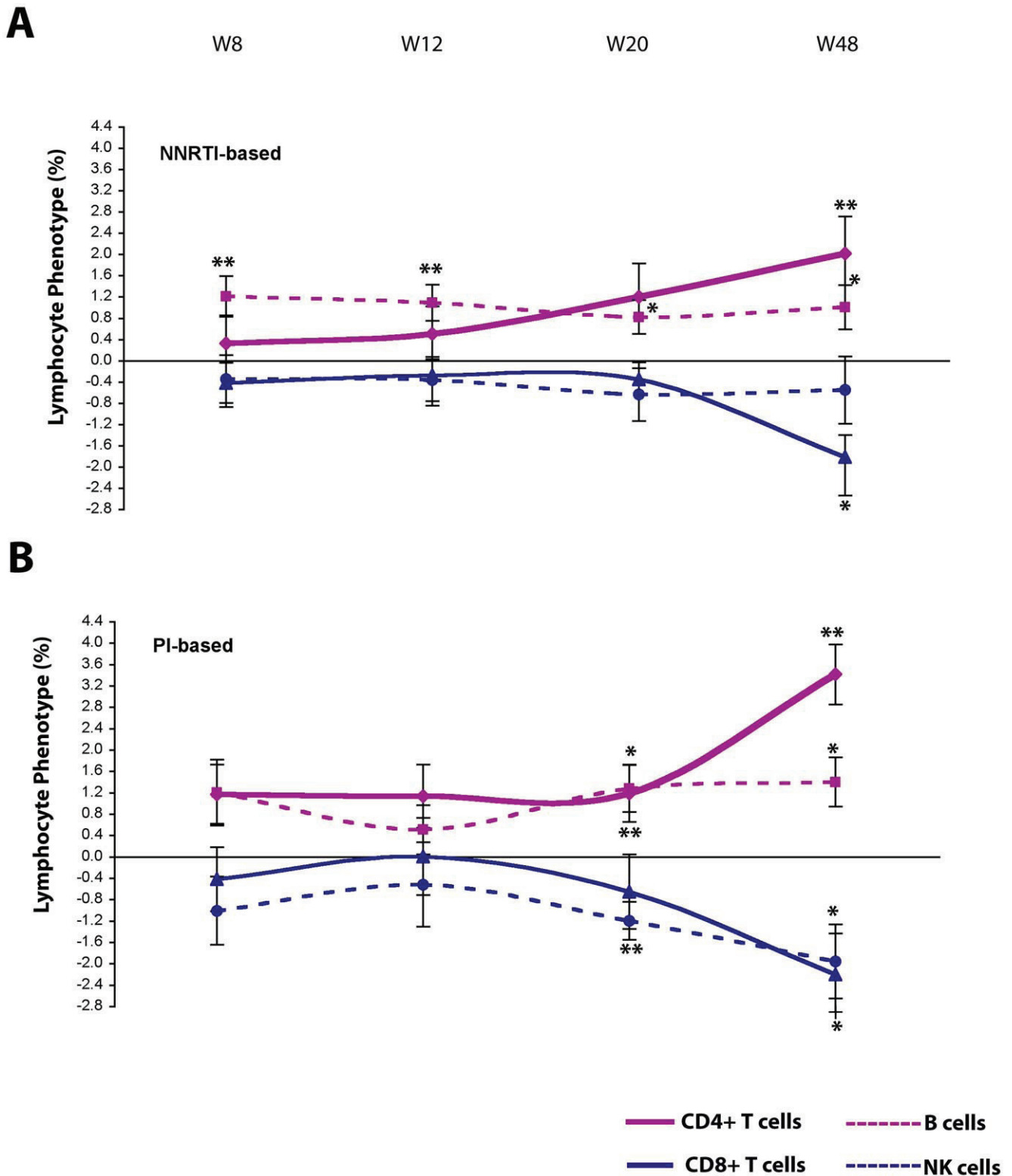
Figure 11. Evaluation of the percentage of CD4 + , CD8 + , NK and B cells in all Tat-immunized subjects after stratification by HAART regimens. Changes from baseline of CD4 + , CD8 + , NK and B cells (percentage) from all immunized patients are shown for NNRTI-based (A) and PI-based (B) treatments. NNRTI-based: n = 51 up to week 20 and n = 41 at week 48; PI-based: n = 19 up to week 20 and n = 12 at week 48, respectively. The t-Test for paired data was used for the analyses: *p < 0.05, **p < 0.01. doi:10.1371/journal.pone.0013540.g011
