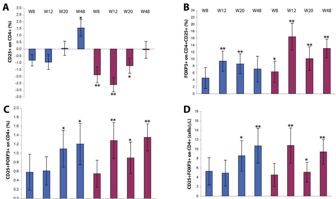
Figure 8. CD25 and FOXP3 expression on CD4 + T cells after Tat immunization. (A) Changes from baseline of CD4 + lymphocytes expressing CD25 are shown according to Tat dose and time after the first immunization (Tat 7.5 \mu g, n = 32 up to week 20 and n = 24 at week 48; Tat 30 \mu g, n = 34 up to week 20 and n = 28 at week 48, respectively). (B) Changes from baseline of the percentage of CD4 + CD25 + lymphocytes expressing FOXP3 + (Tat 7.5 \mu g, n = 31 up to week 20 and n = 23 at week 48; Tat 30 \mu g, n = 29 up to week 20 and n = 28 at week 48, respectively). (C) Changes from baseline of the percentage of CD4 + T cells expressing CD25 + FOXP3 + (Tat 7.5 \mu g, n = 31 up to week 20 and n = 23 at week 48; Tat 30 \mu g, n = 29 up to week 20 and n = 24 at week 48). (D) Changes from baseline of the absolute number of CD4 + lymphocytes expressing CD25 + FOXP3 + (Tat 7.5 \mu g, n = 30 up to week 20 and n = 20 at week 48; Tat 30 \mu g, n = 29 up to week 20 and n = 22 at week 48, respectively). Blue bars: Tat 7.5 \mu g; red bars: Tat 30 \mu g. Data are presented as the mean changes ( \pm standard error) evaluated at 8, 12, 20 and 48 weeks after the first immunization. The t-Test for paired data was used for the analyses: * p < 0.05 , ** p < 0.01 . doi:10.1371/journal.pone.0013540.g008
