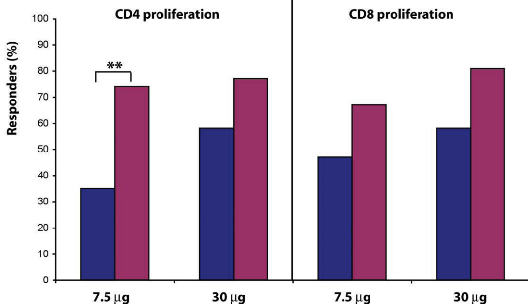
Figure 3. Anti-Tat cellular immune responses. (A) Percentage of subjects showing anti-Tat specific production of IFN- \gamma , IL-2 or IL-4, respectively, measured at baseline (blue bar) and up to week 48 after the first immunization (red bar) and stratified by Tat dose (Tat 7.5 \mu g, n = 35; Tat 30 \mu g, n = 33 subjects, respectively). (B) Percentage of subjects showing anti-Tat CD4^+ or CD8^+ lymphoproliferative responses measured at baseline and up to week 48 and stratified by Tat dose (Tat 7.5 \mu g, n = 31; Tat 30 \mu g, n = 31). The analysis was performed using the McNemar's test: * p < 0.05 , ** p < 0.01 . doi:10.1371/journal.pone.0013540.g003
