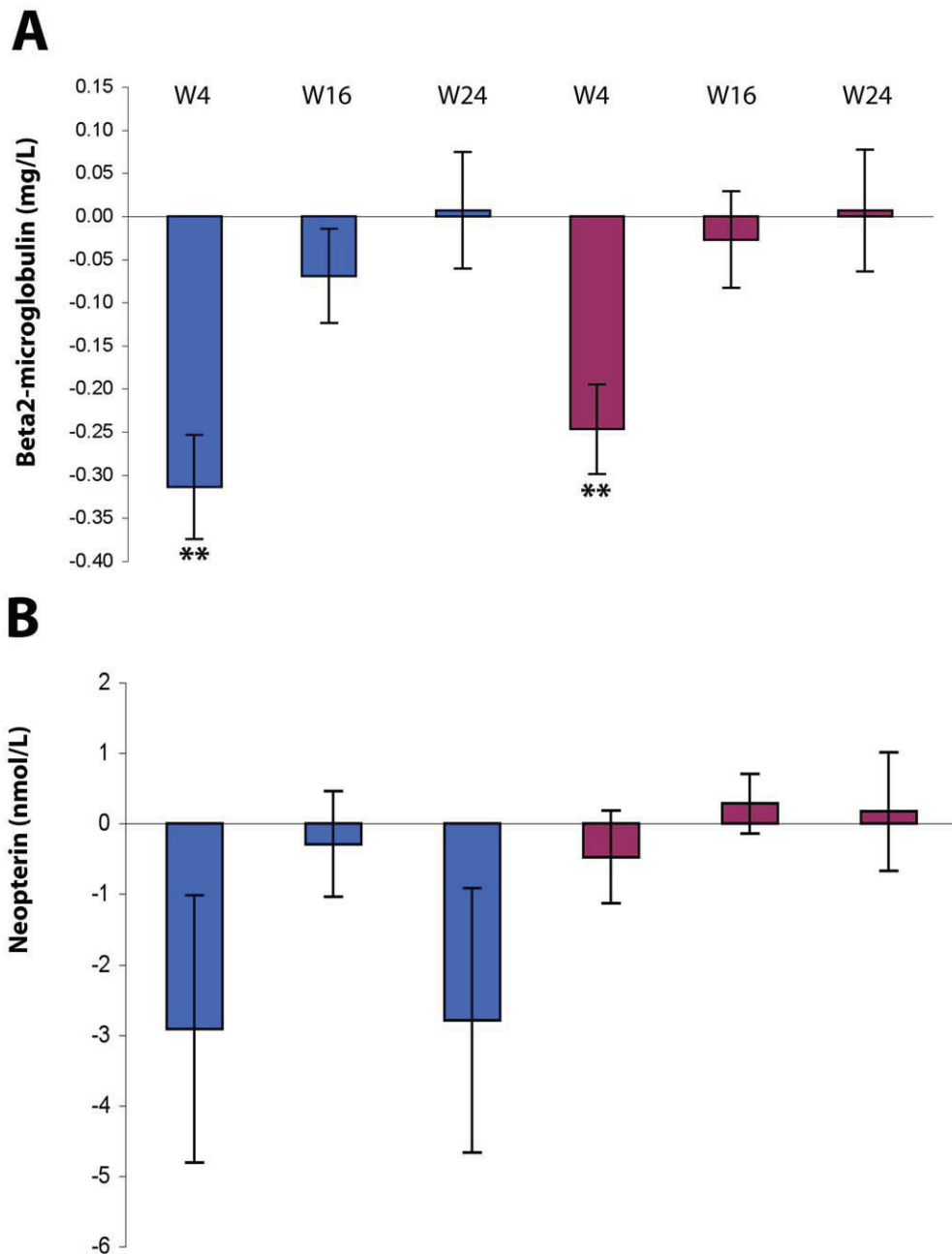
Figure 6. Production of \beta 2-microglobulin and neopterin after Tat immunization. Changes from baseline, according to Tat dose, of (A) \beta 2-microglobulin serum levels (mg/L) and (B) Neopterin (nmol/L). Blue bars: Tat 7.5 \mu g; red bars: Tat 30 \mu g. Data are presented as the mean changes ( \pm standard error) at 4, 16 and 24 weeks (Tat 7.5 \mu g, n = 37, Tat 30 \mu g, n = 40 subjects, respectively). The t-Test for paired data was used for the analyses: **p < 0.01. doi:10.1371/journal.pone.0013540.g006
