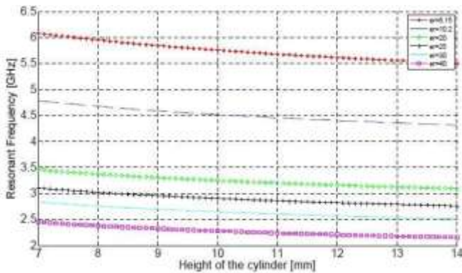
Figure 2: Graph of resonant frequencies for TM 01 mode
