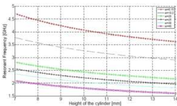
Figure 3: Graph of resonant frequencies for HE 11 mode
