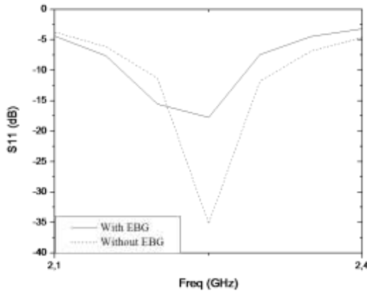
Figure 5: Simulated return loss of the proposed antenna
