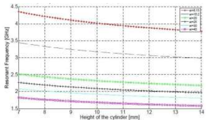
Figure 1: Graph of resonant frequencies for TE 01 mode
