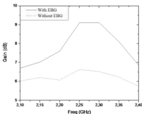
Figure 6: Simulated gain of the proposed antenna
