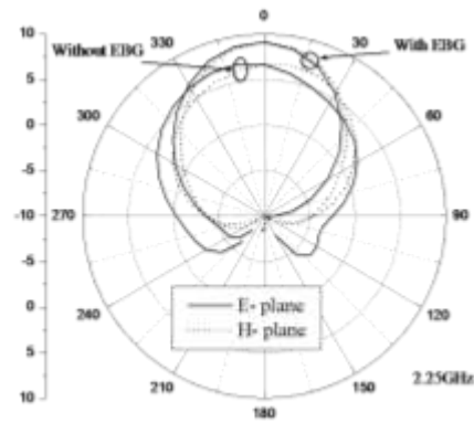
Figure 7: Simulated radiation pattern of the proposed antenna
