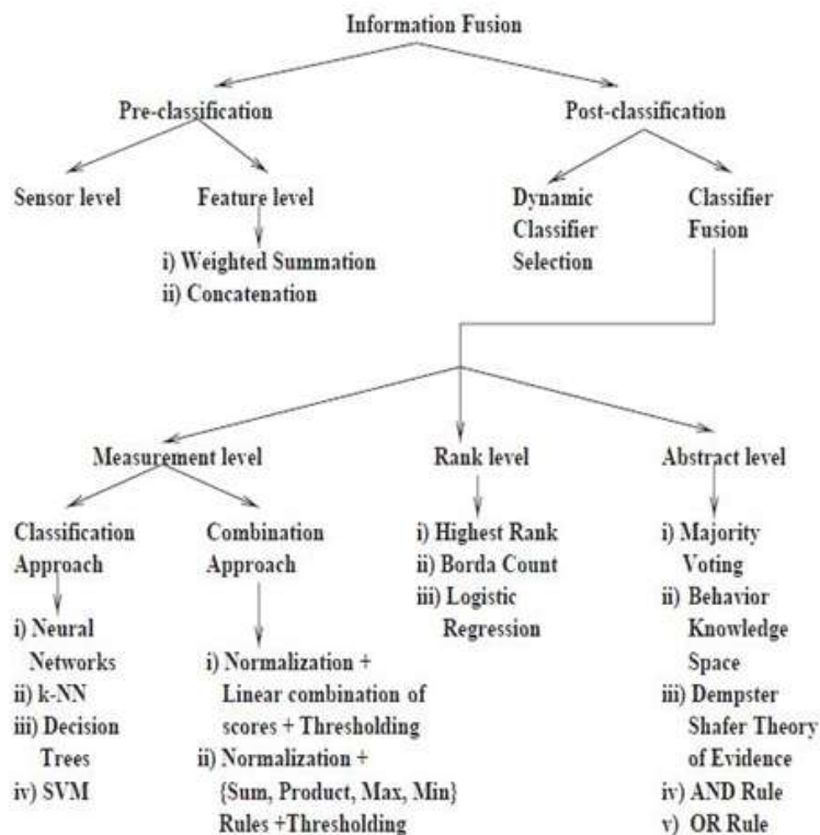
.Fig. 4 Approaches to information fusion
