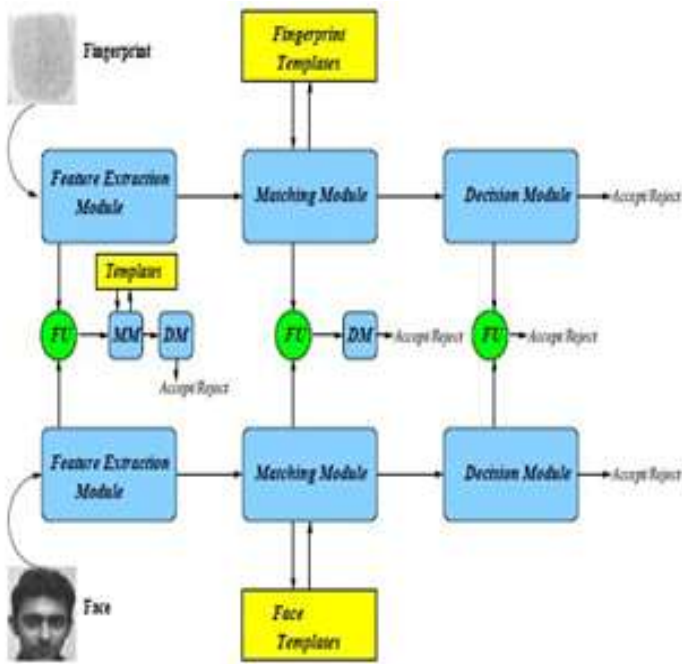
Fig. 5 Levels of fusion in bimodal biometric system; FU: Fusion Module, MM: Matching Module, DM: Decision Module
