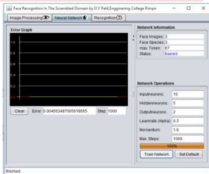
Fig.2 Error Graph
