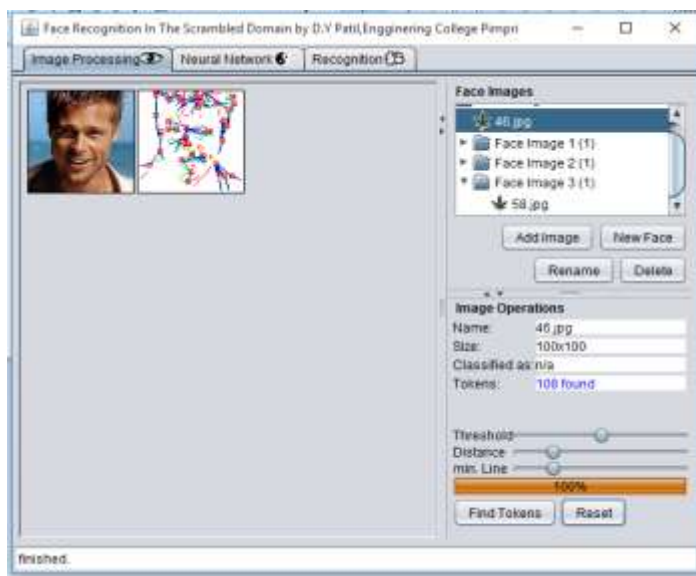
Fig.1 Image Processing
