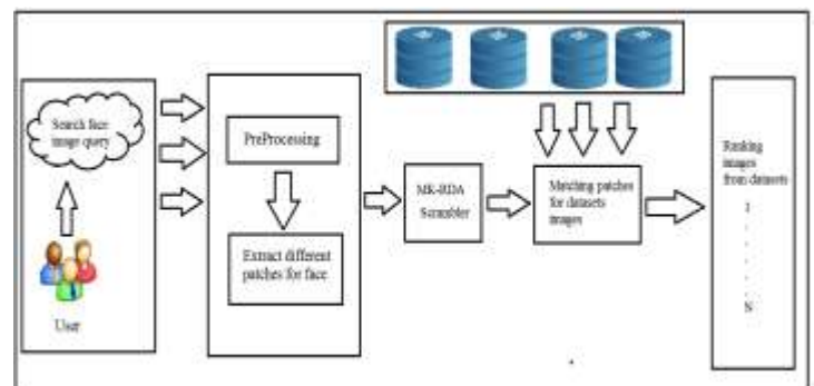
Fig1. System Architecture.
