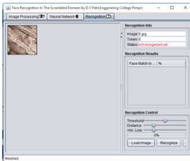
Fig.3 Recognition
