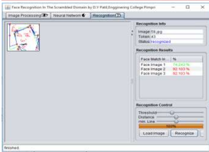
Fig.4 Matching Accuracy
