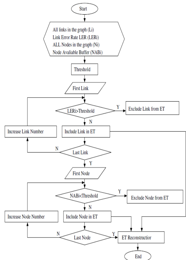
Figure 1. Flowchart of SSRA.
