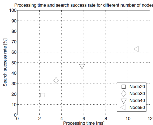
Figure 3. Relation between processing time and search success rate
