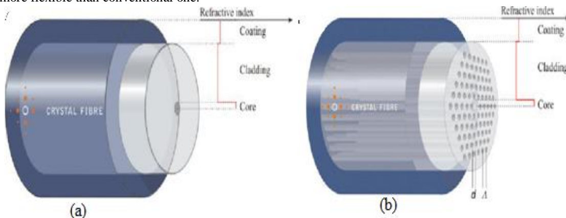
Fig.1 (a) A Standard optical fiber (b) A Photonic crystal fiber
