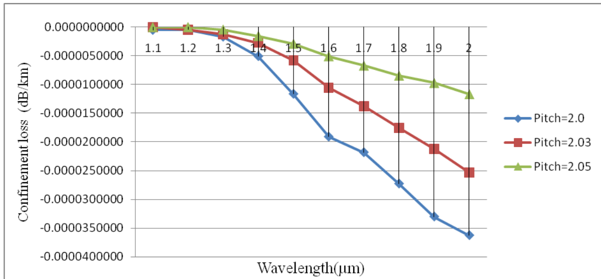
Fig. 10 Confinement loss with wavelength (Design-3 at different Pitch)
