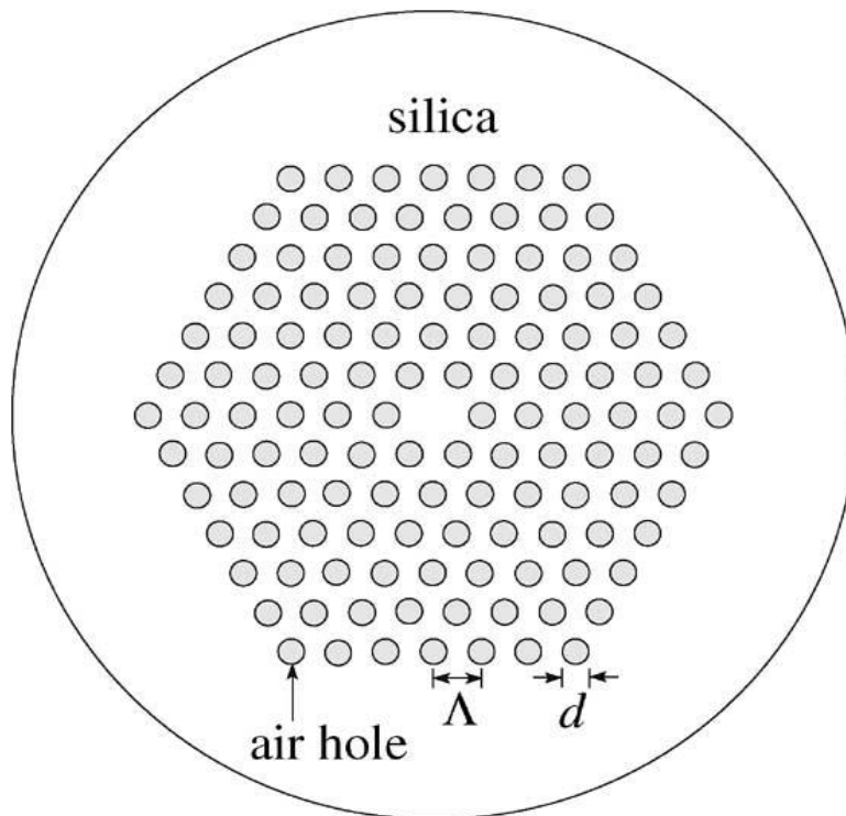
Fig.2 Photonic crystal fiber representation
