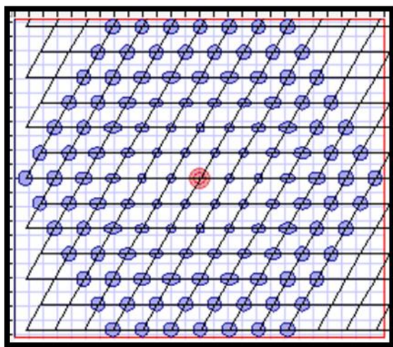
Fig. 6 Cross section of proposed PCF at pitch=2.05µm
