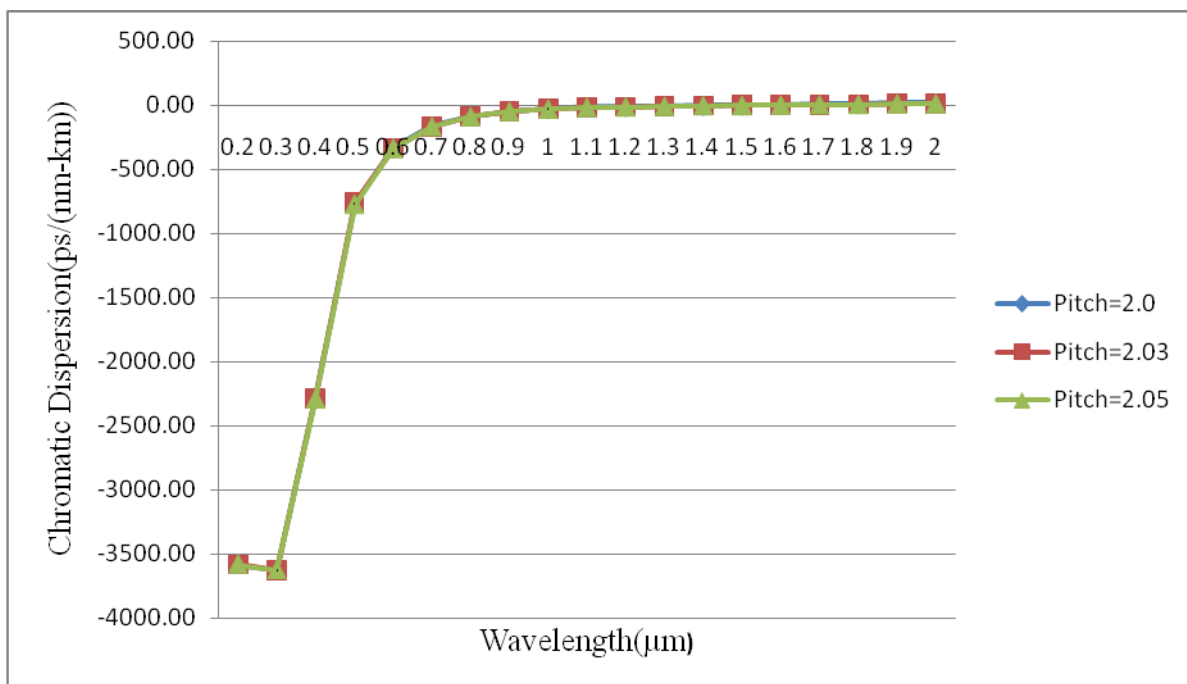
Fig. 9 Chromatic dispersion of PCF Design at different pitch
