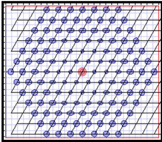
Fig. 5 Cross section of proposed PCF at pitch=2.03µm
