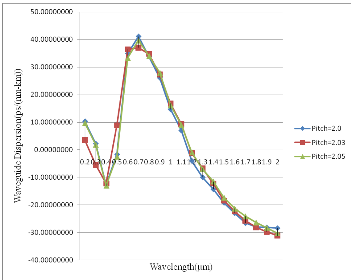
Fig. 8 Waveguide dispersion with wavelength
