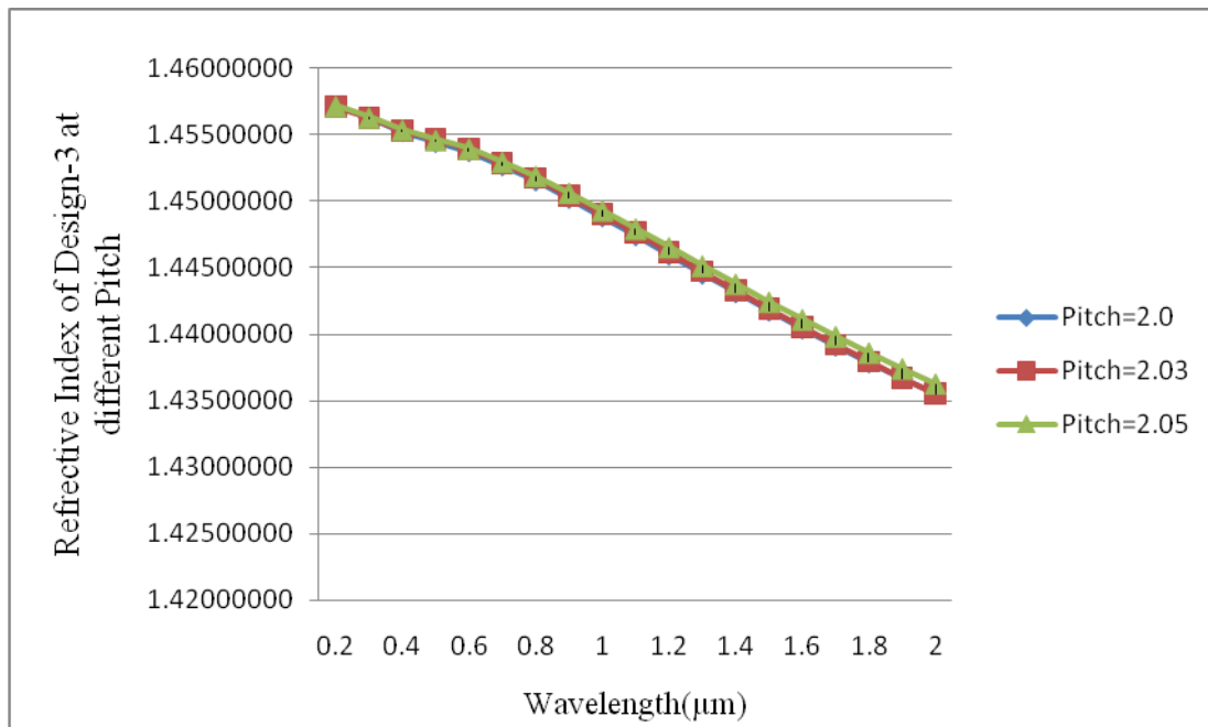
Fig. 7 Effective Refractive index
