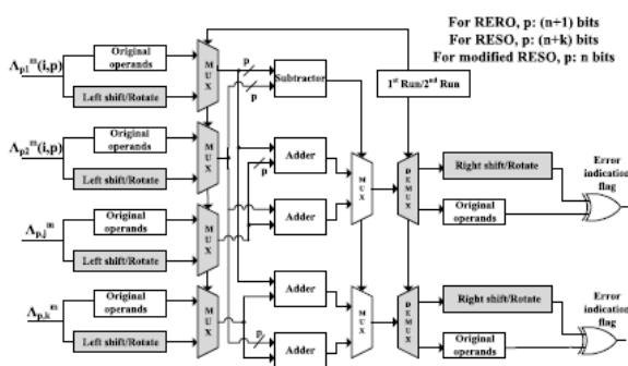
Figure 2. PCSA error detection through re computing with encoded operands.
