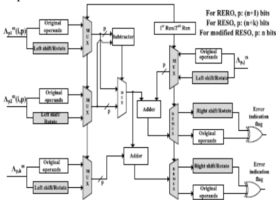
Figure 1. Re computing with encoded operands for CSA
