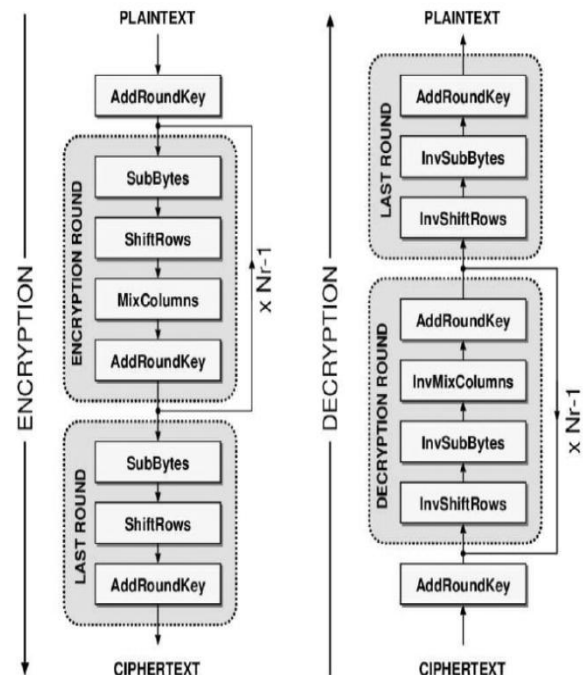
Fig: Working of AES algorithm
