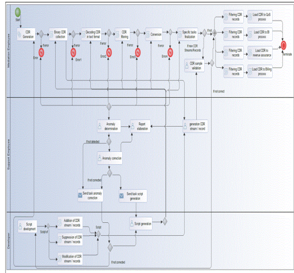
Figure 6. BPMN process diagram of mediation before application of ISPM
