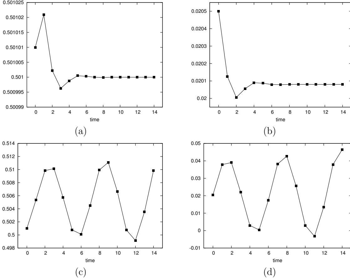
Figure 5: Trajectories for systems perturbed away from equilibrium. When the function f(r) = 0.5 + 0.0498r and the fixed point (0.501, 0.02) are considered, both \pi (panel a) and r (panel b) stabilize through the oscillations. For the function f(r) = 0.5 + 0.26r the oscillations of \pi (panel c) and r (panel d) around the fixed point (0.505, 0.02) are reinforcing and the system does not stabilize. In both cases is \bar{\epsilon} = 0.02 .
