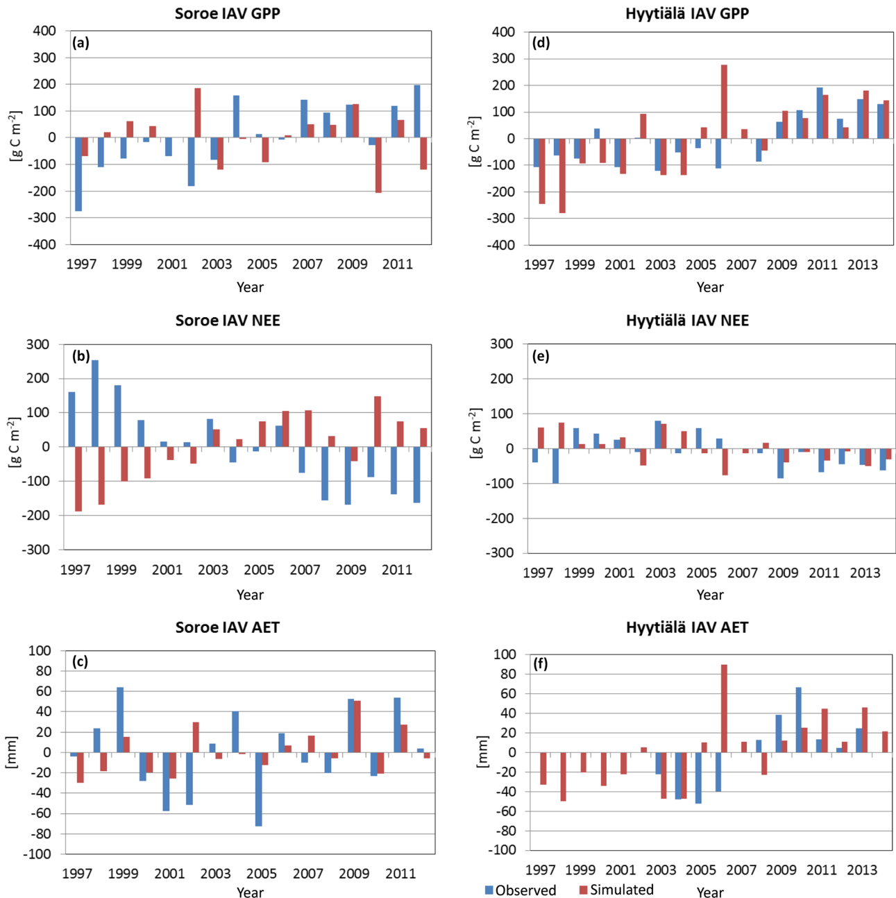
Figure 7. Inter-annual variability (IAV) of GPP, NEE, and AET (sim – simulated and obs – observed) in Sorø (a–c) and Hyttiälä (d–f).
