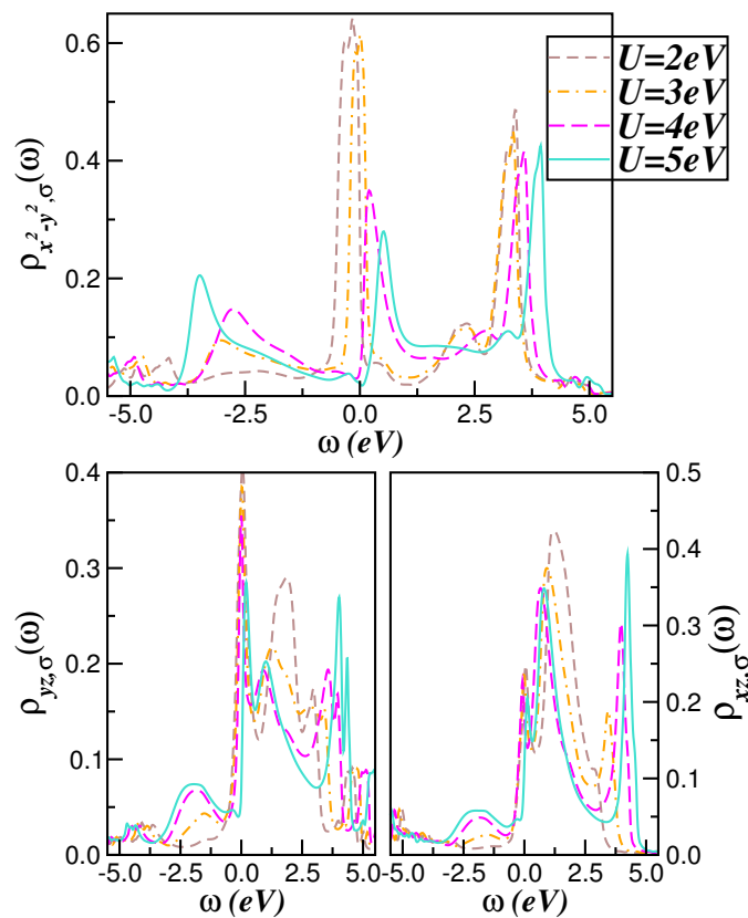
Figure 3. Effect of electronic correlations on the orbital-resolved LDA+DMFT density-of-states (DOS) of monoclinic \text{MoO}_2 . Worth noticing is the dynamical evolution of the d_{x^2-y^2} bonding-antibonding branch, which shows an overall shift to energies above E_F due to correlation-induced spectral weight transfer. Also relevant is the formation of a pseudogap-like state at energies near the Fermi level ( E_F = \omega = 0.0 ) for U = 5 eV.
