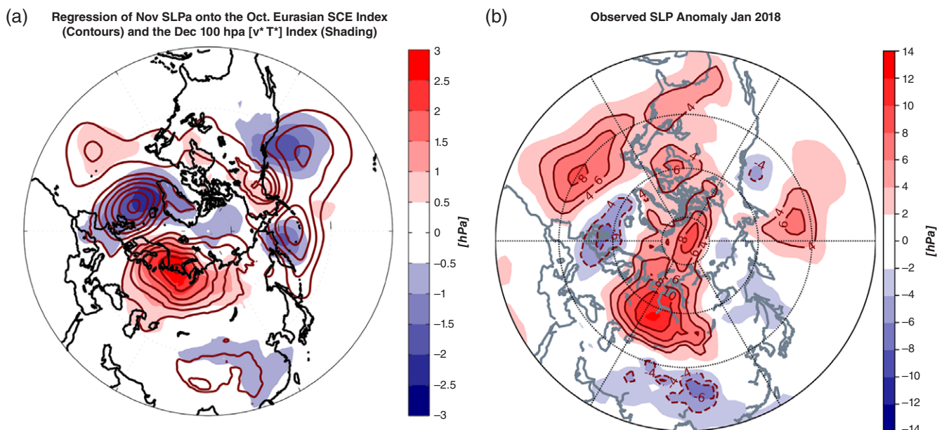
FIGURE 6 (a) Regression of November sea level pressure (SLP) anomalies (hPa) onto October monthly mean Eurasian snow cover extent (contouring) and onto December meridional heat flux anomalies at 100 hPa, averaged between 40°N and 80°N (shading). This figure is the same as fig. 4 from Cohen, Furtado, et al. (2014). (b) Observed mean SLP (contours) and SLP anomalies (shading) for January 2018
