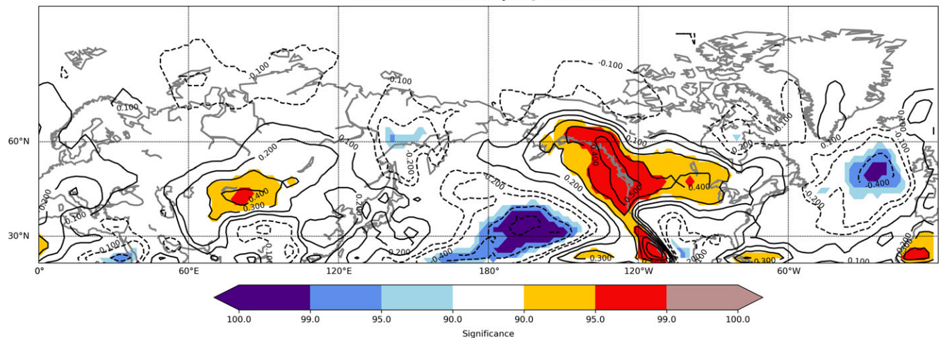
FIGURE 5 Correlation of Niño 3.4 index with surface temperatures across the Northern Hemisphere (contouring). Correlation of 90, 95 and 99% are represented by light, dark and darkest shading, respectively. Red shading represents positive correlations and blue shading represents negative correlations
