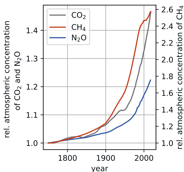
Fig. 1. Atmospheric abundances of the greenhouse gases CO 2 , CH 4 , and N 2 O, shown relative (rel.) to their pre-industrial levels in 1750: CO 2 at 270 ppm, CH 4 at 719.01 ppb, N 2 O at 270 ppb. Data provided by the European Environment Agency (EEA). [2] The current levels are stated in Table 1.
