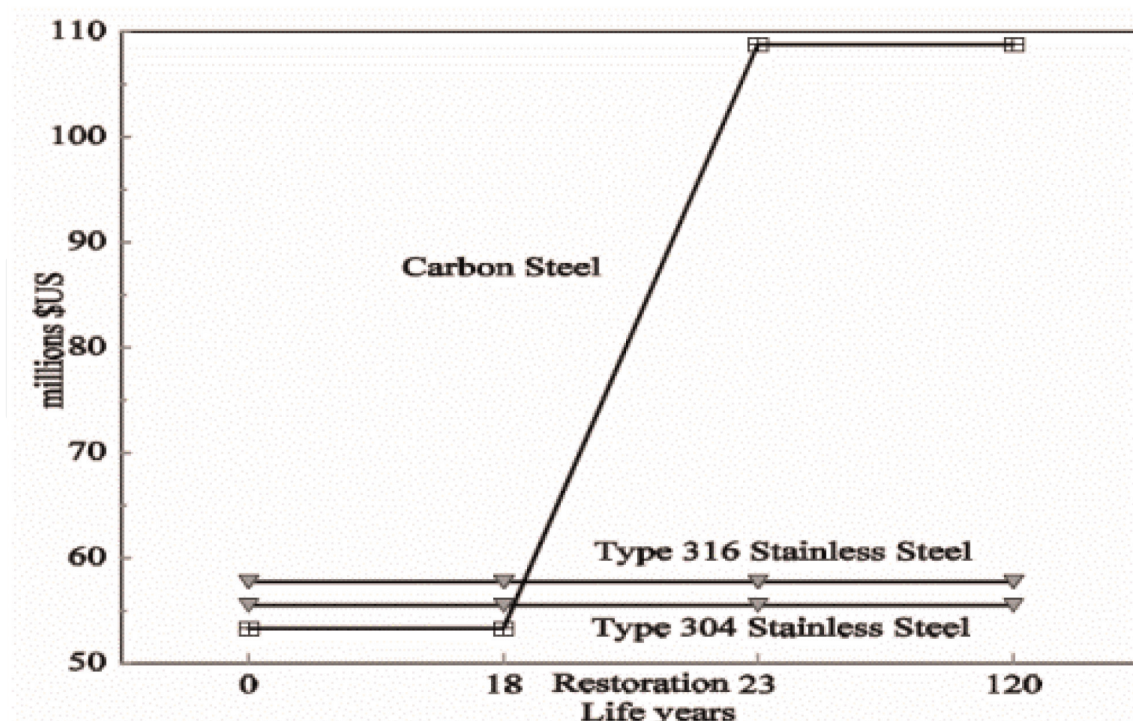
Figure 2. Life cycle cost analysis for Sweden's Oland bridge [17].
