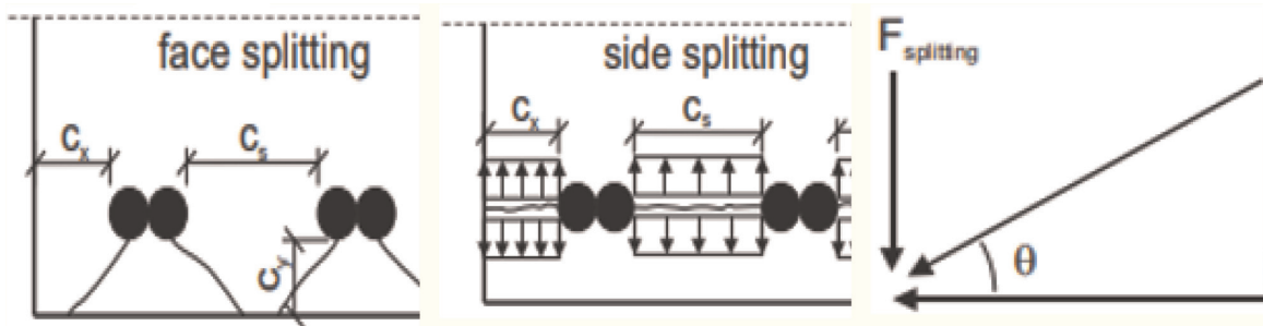
Figure 12. Face splitting (left), side splitting (middle) and force distribution at bond forces (right). [Adapted from [47]].
