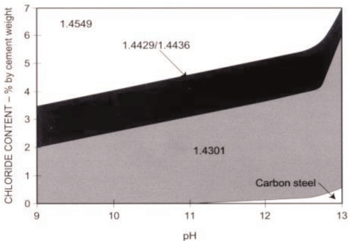
Figure 8. Corrosion performance of various stainless steel compared to carbon steel [34].
