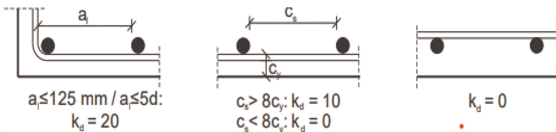
Figure 10. Coefficient k_d for efficiency of stirrups (Source: [37]).
