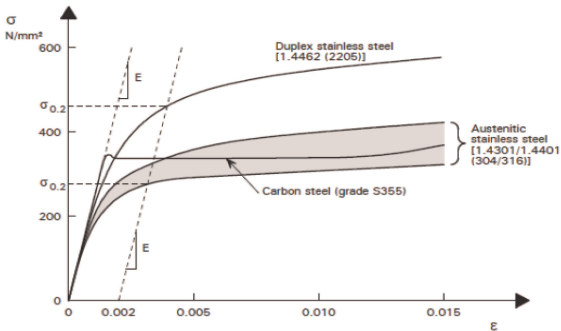
Figure 1. Stress-strain curves for stainless steel and carbon steel [7].
