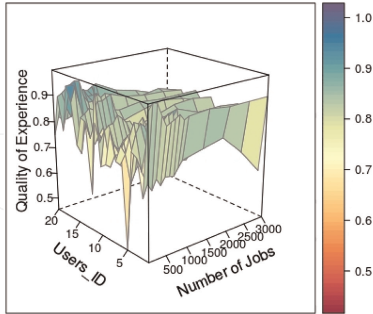
Figure 2. QoE per user Round Robin and Dijkstra.
