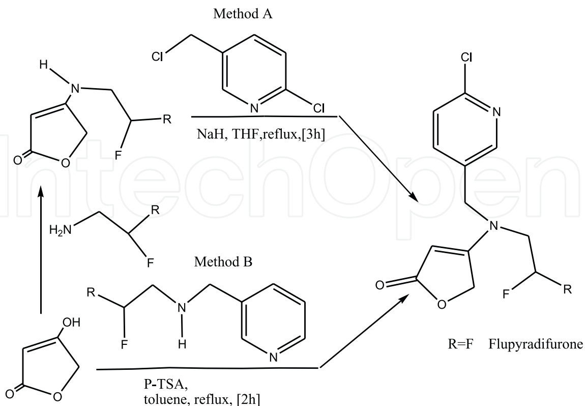
Figure 15. Flupyradifurone synthesis.
