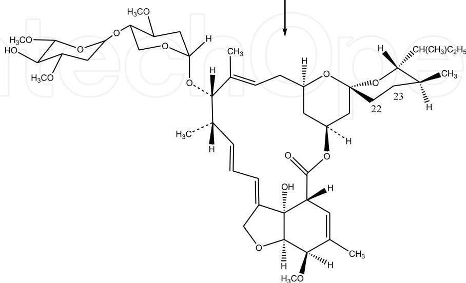
22,23-dihydroavermectin A 1
