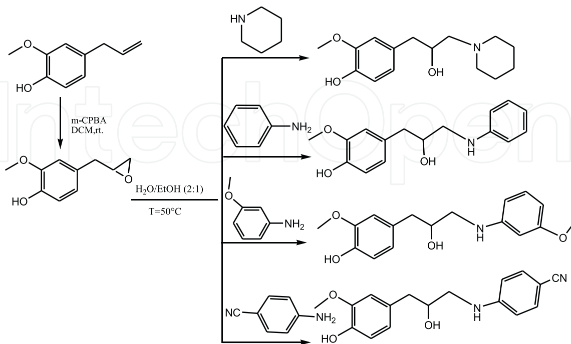
Figure 17. Hemisynthesis of eugenol alcohols.
