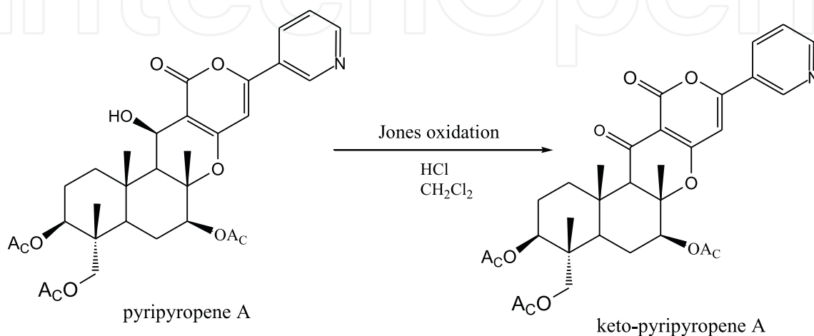
Figure 8. Keto-pyripyropene A synthesis [45].
