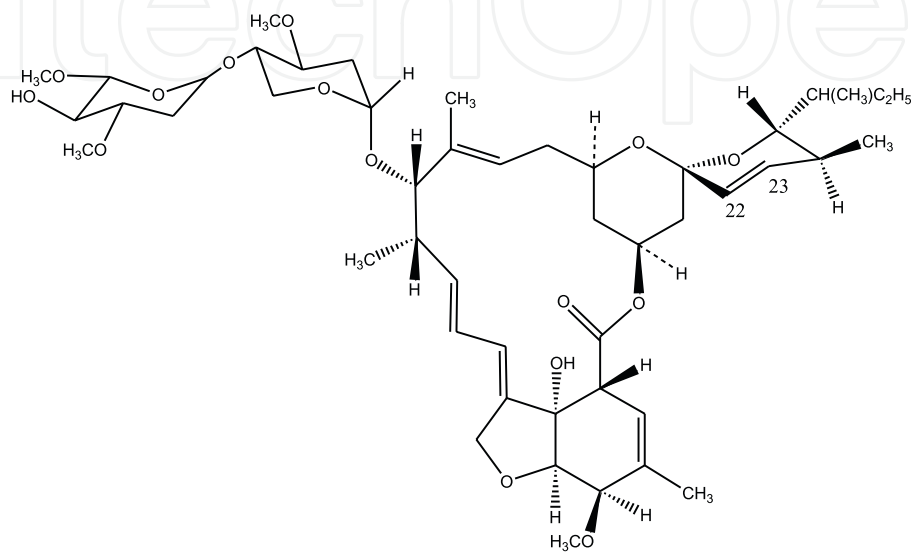
avermectin A 1
