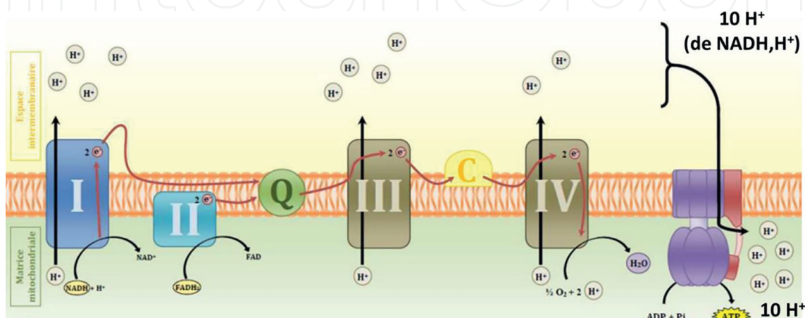
Figure 29. Electron transport chain [108].
