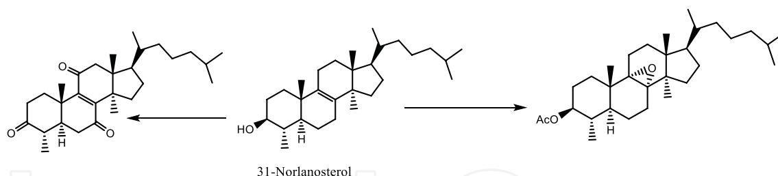
Figure 28. Triterpenic derivatives synthesis.
