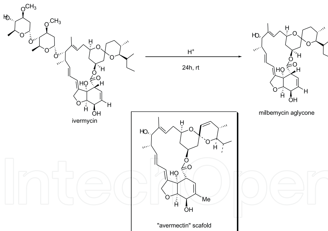
Figure 4. Milbemycin aglycone synthesis [32].
