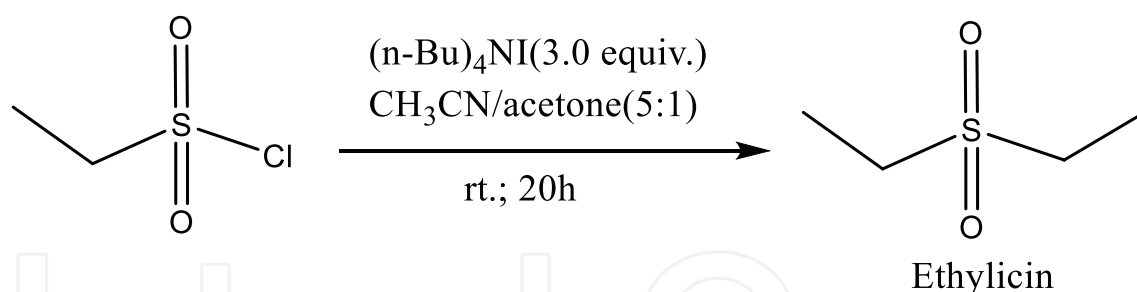
Figure 26. Ethylsulfonate synthesis.
