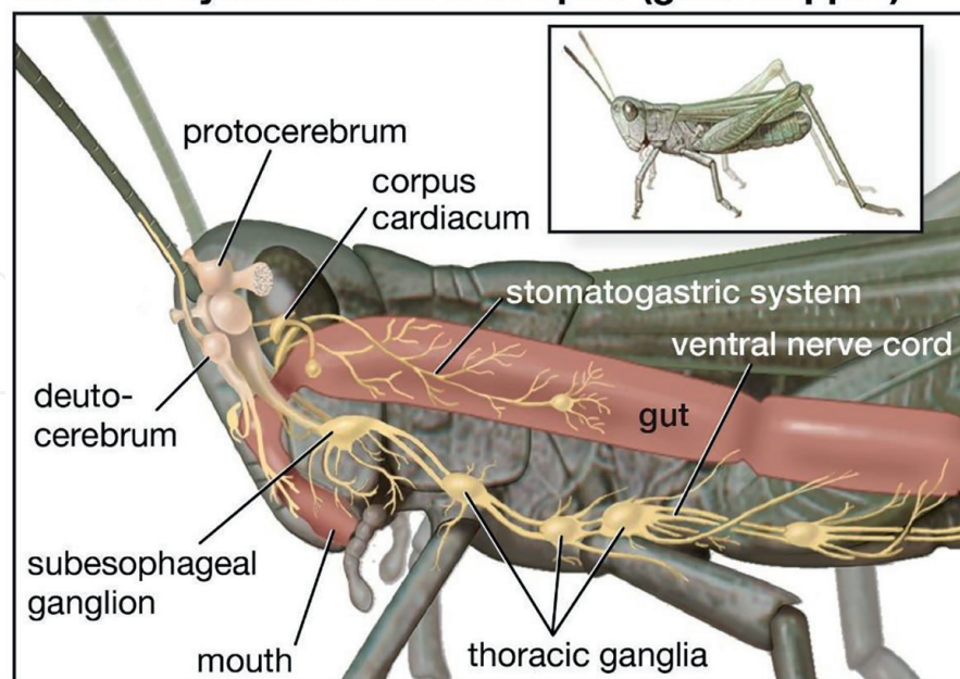
Figure 2. Nervous system of the grasshopper [27].
