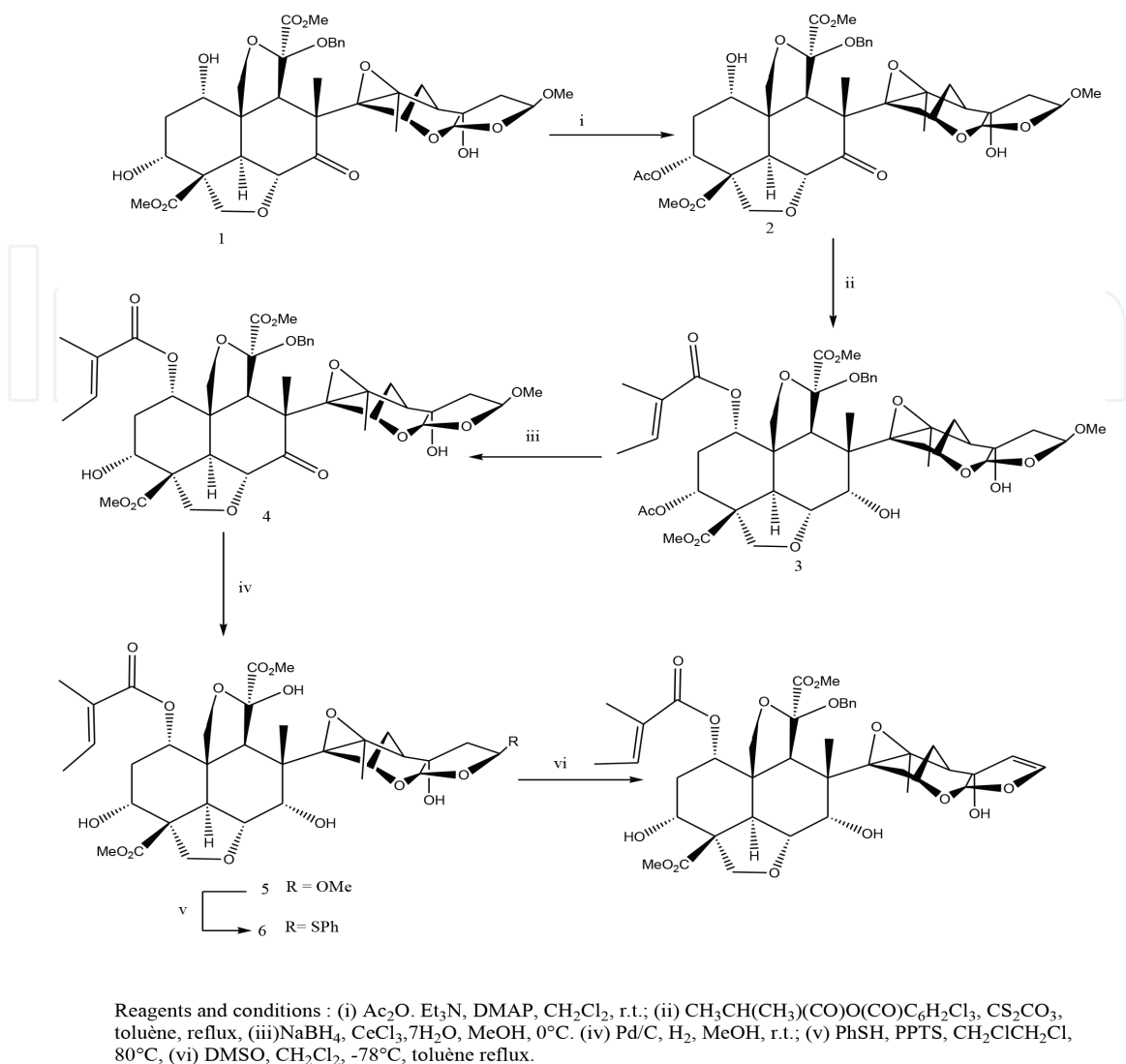
Figure 19. Azadirachtin synthesis.
