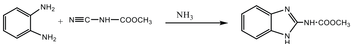
Figure 25. Carbendazim synthesis.
