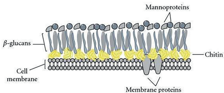
Figure 20. Fungal cell wall components [82].
