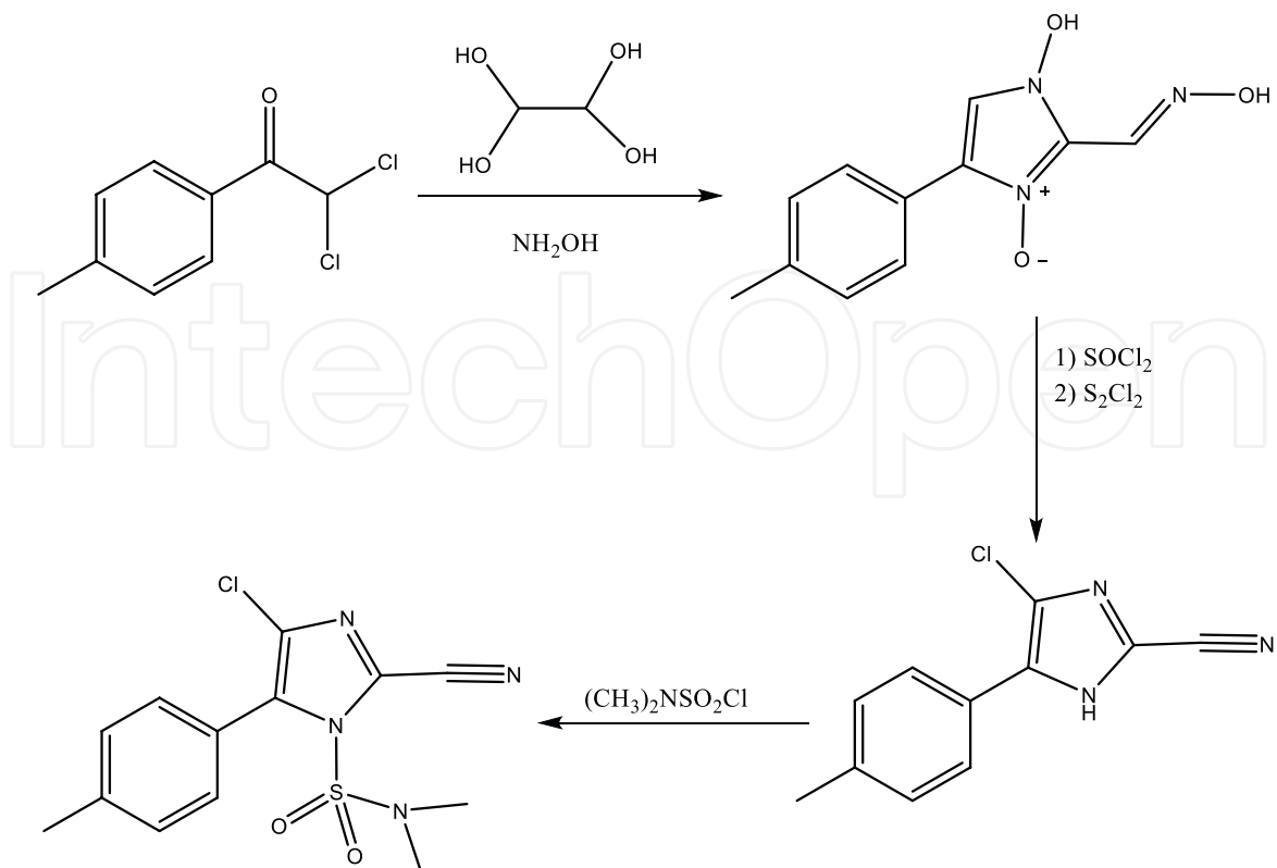
Figure 30. Cyazofamid synthesis.
