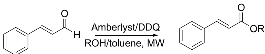
Figure 13. Hemisynthesis of phenylpropanoids derivatives.
