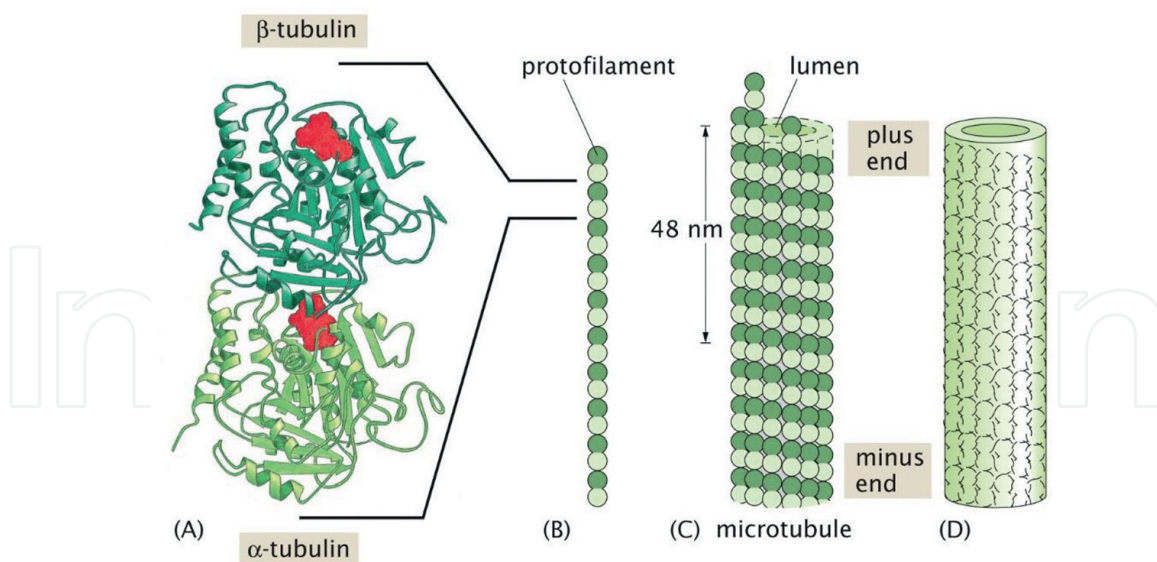
Figure 24. Microtubules formation: A. Tubulin dimerization; B. Tubulin dimers polymerization; C. Protofilament association; D. Formed microtubule [90].
