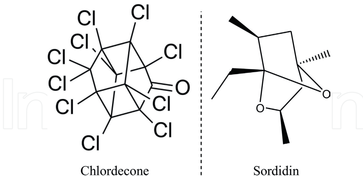
Figure 1. Chlordecone (left) and sordidin (right) structures.
