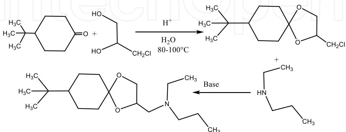
Figure 22. Spiroxamine synthesis.
