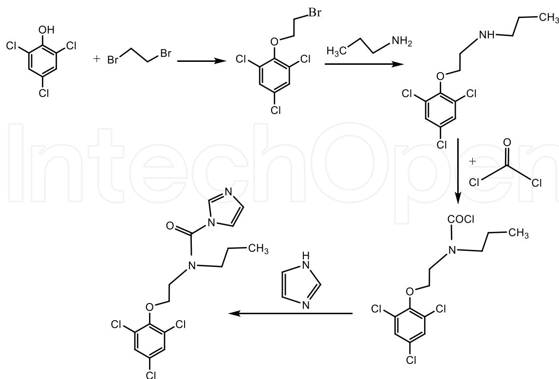
Figure 23. Prochloraz synthesis.
