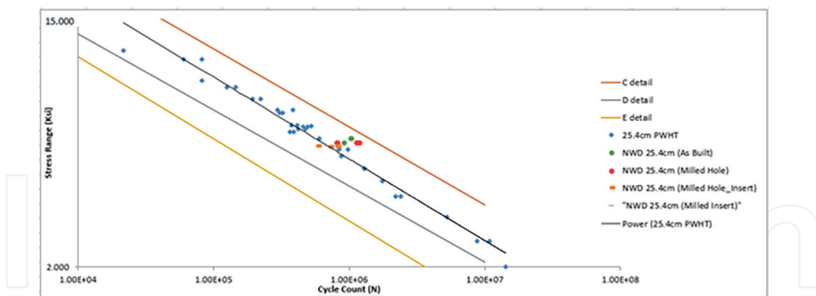
Figure 7. New weld detail vs. old 10in data.
