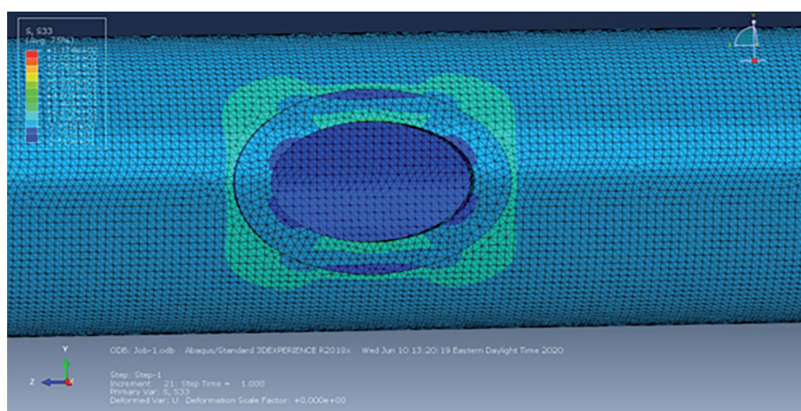
Figure 12. Contours of longitudinal stresses around the hand-holes.
