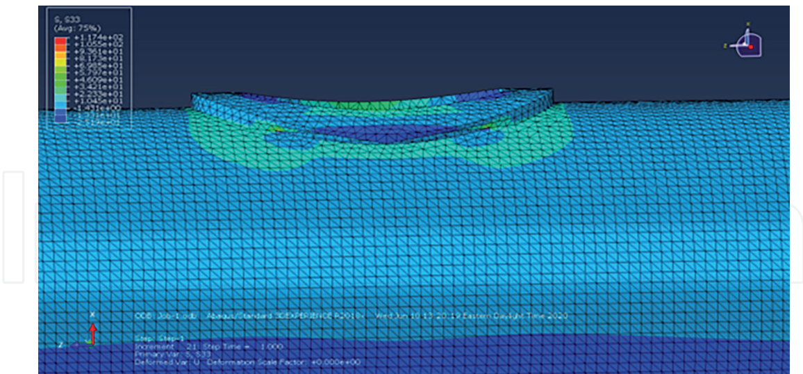
Figure 14. Stress concentration Z direction.
