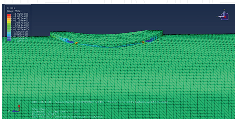
Figure 13. Stress concentration X direction.
