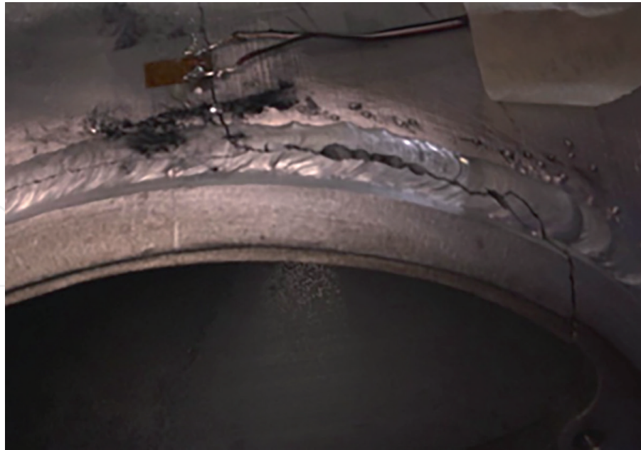
Figure 10. Typical final failure of hand-hole details.
