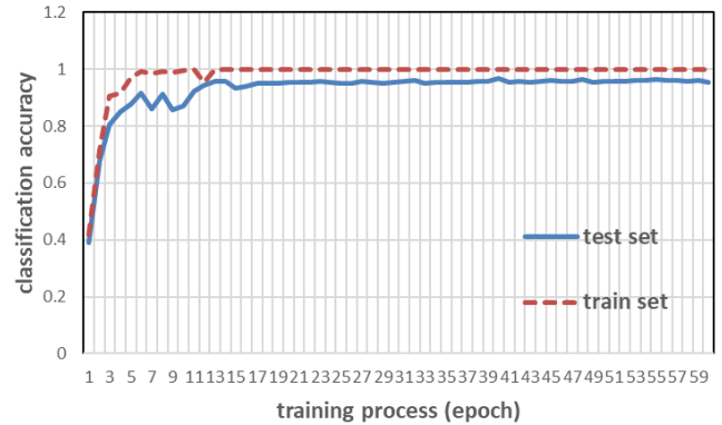
Fig.4 The measurement of classification accuracies on training set and test set as the training process is going on: classifier 3
