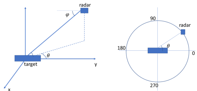
Fig.1 Geometry of SAR and top view of aspect angles: \varphi is depression angle and \theta is aspect angle, \varphi=15^\circ, 17^\circ, 30^\circ, 44^\circ . \theta was sampled from 0 to 360 for each depression angle. Images for \varphi=17^\circ are used for training set while \varphi=15^\circ for test set.
