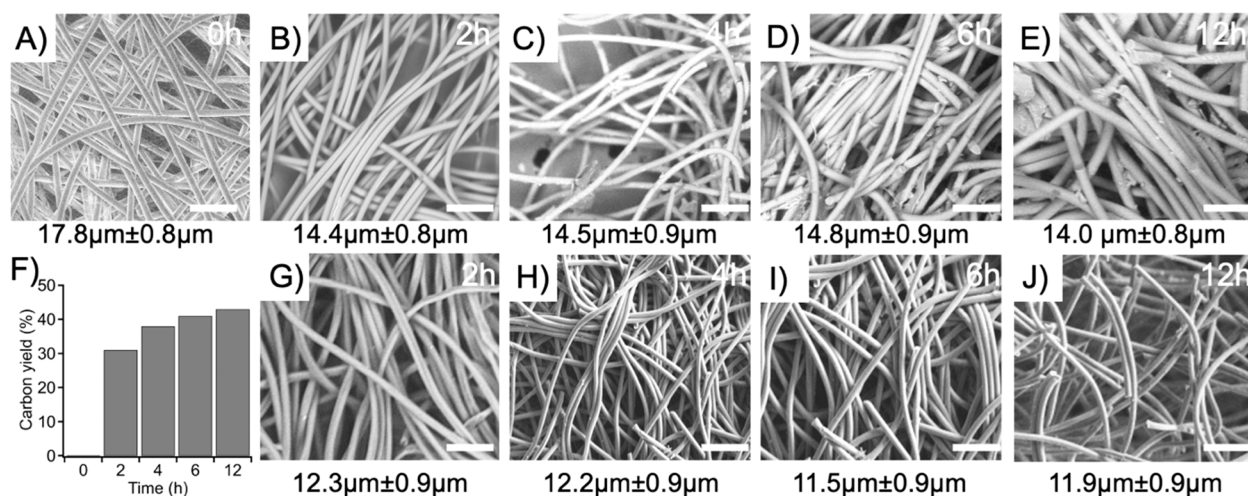
Figure 2. (A) SEM images of mask-derived PP fibers and after cross-linking for (B) 2, (C) 4, (D) 6, and (E) 12 h. (F) Carbon yield of PP fibers with an increasing crosslinking time. SEM images of carbon fibers with cross-linking times of (G) 2, (H) 4, (I) 6, and (J) 12 h. Scale bar of 100 μm.
