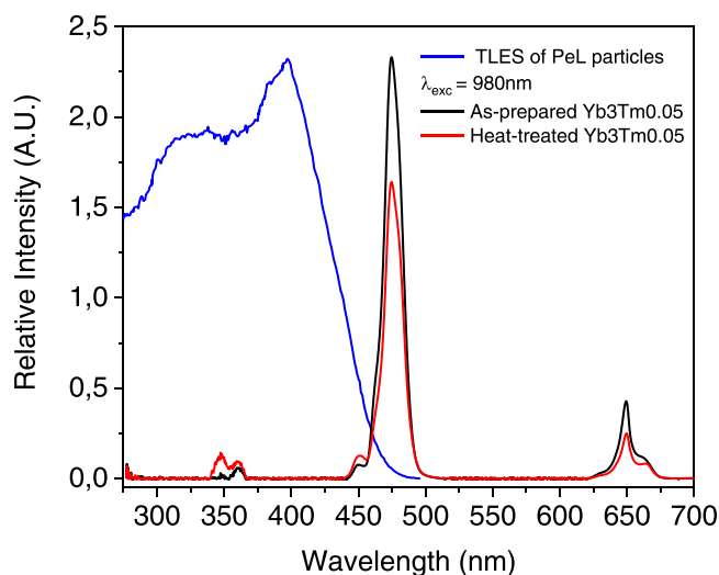
Fig. 9. UC emission spectra of the Yb3Tm0.05 glass prior to and after heat treatment and thermoluminescence excitation spectrum (TLES) of the PeL particles, taken from [39].
