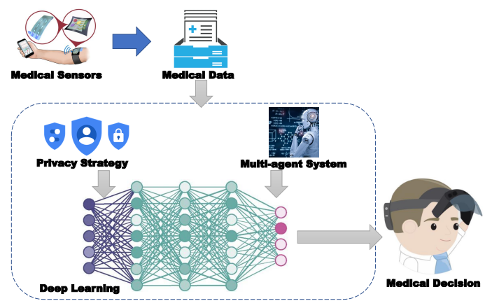
Fig. 1. SCF-BHI Framework
