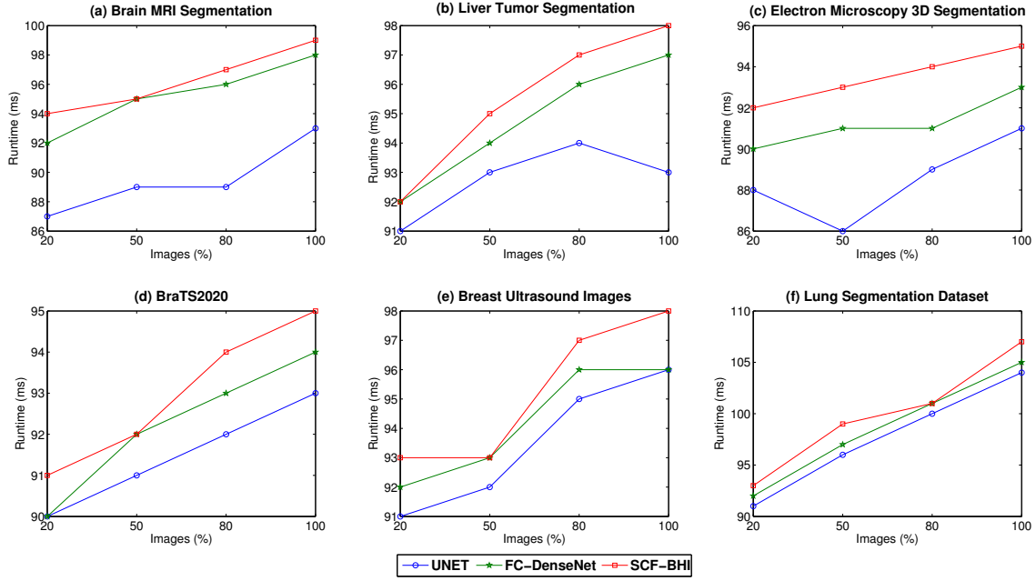
Fig. 4. Runtime of the SCF-BHI compared to the state-of-the-art image segmentation solutions.
