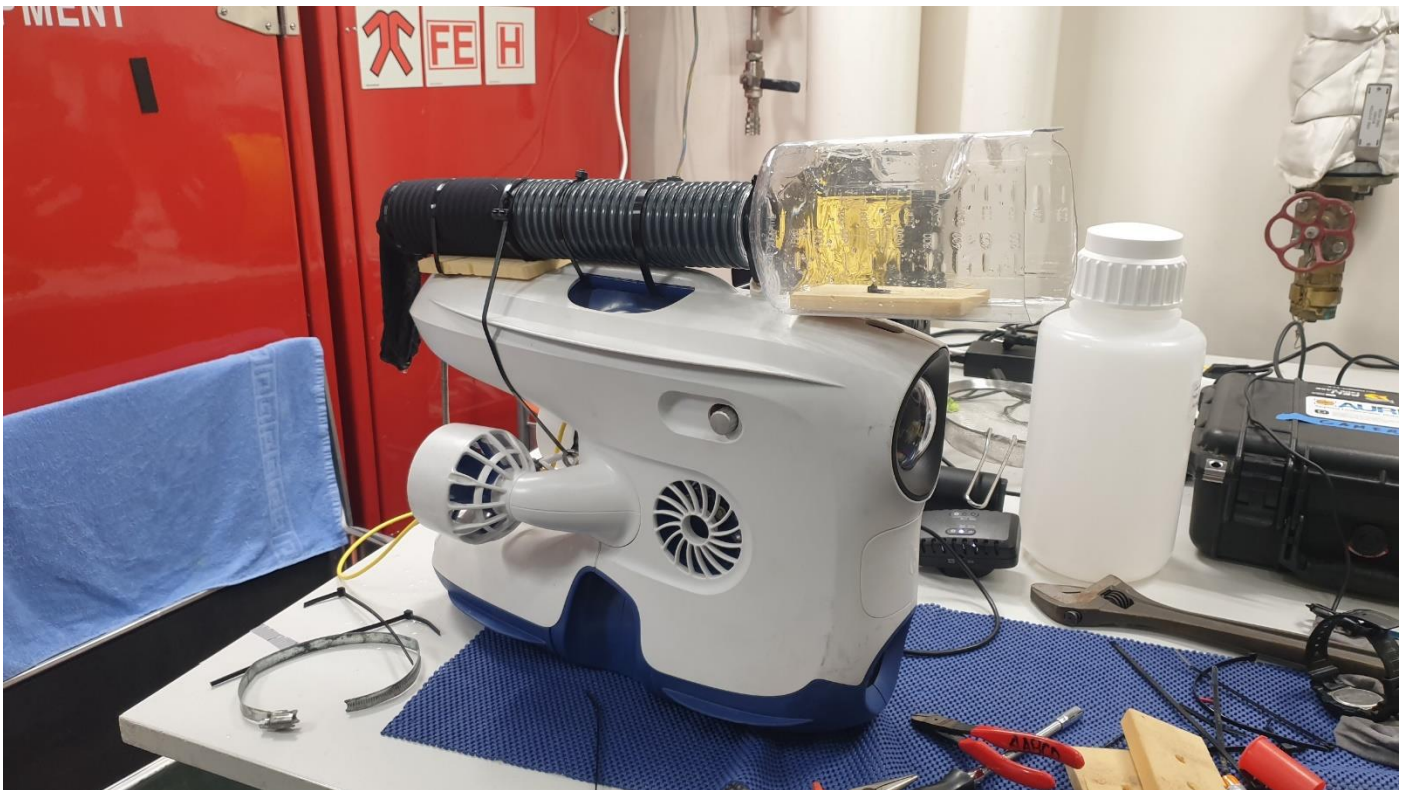
Figure 57. The Blueeye was equipped with an improvised sampling mechanism with the hope that it could collect algae samples. The one shown is the 2nd of four different devices built in total.
