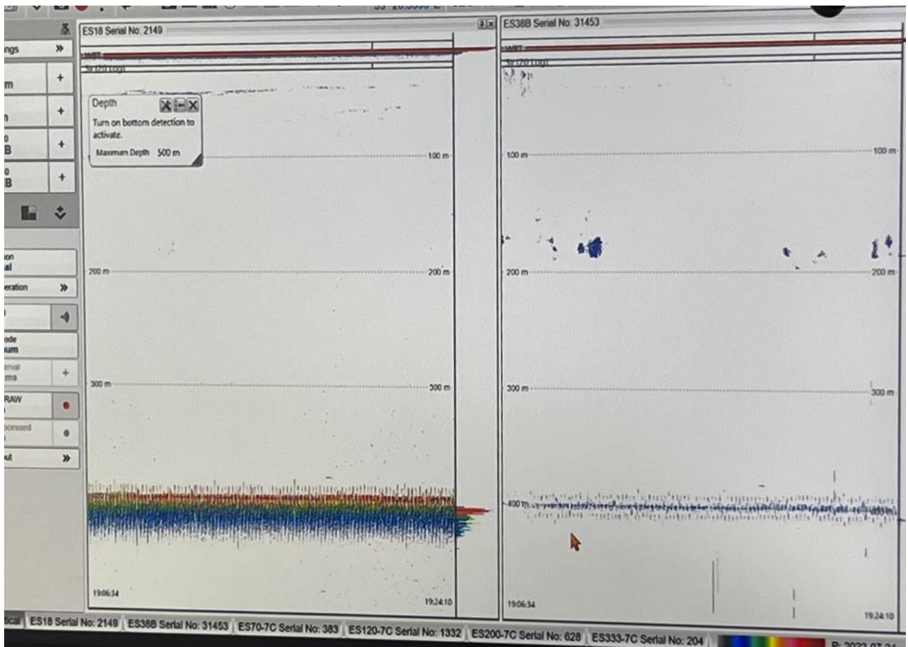
Figure 17. Krill swarms about 180 m depth recorded on the 38 kHz channel (right) at the Simrad EK80 echo sounder at TR-3, 23 July 2022. But no recordings of these swarms at the 18 kHz channel. False bottom detection on both channels at 400 m depth.
