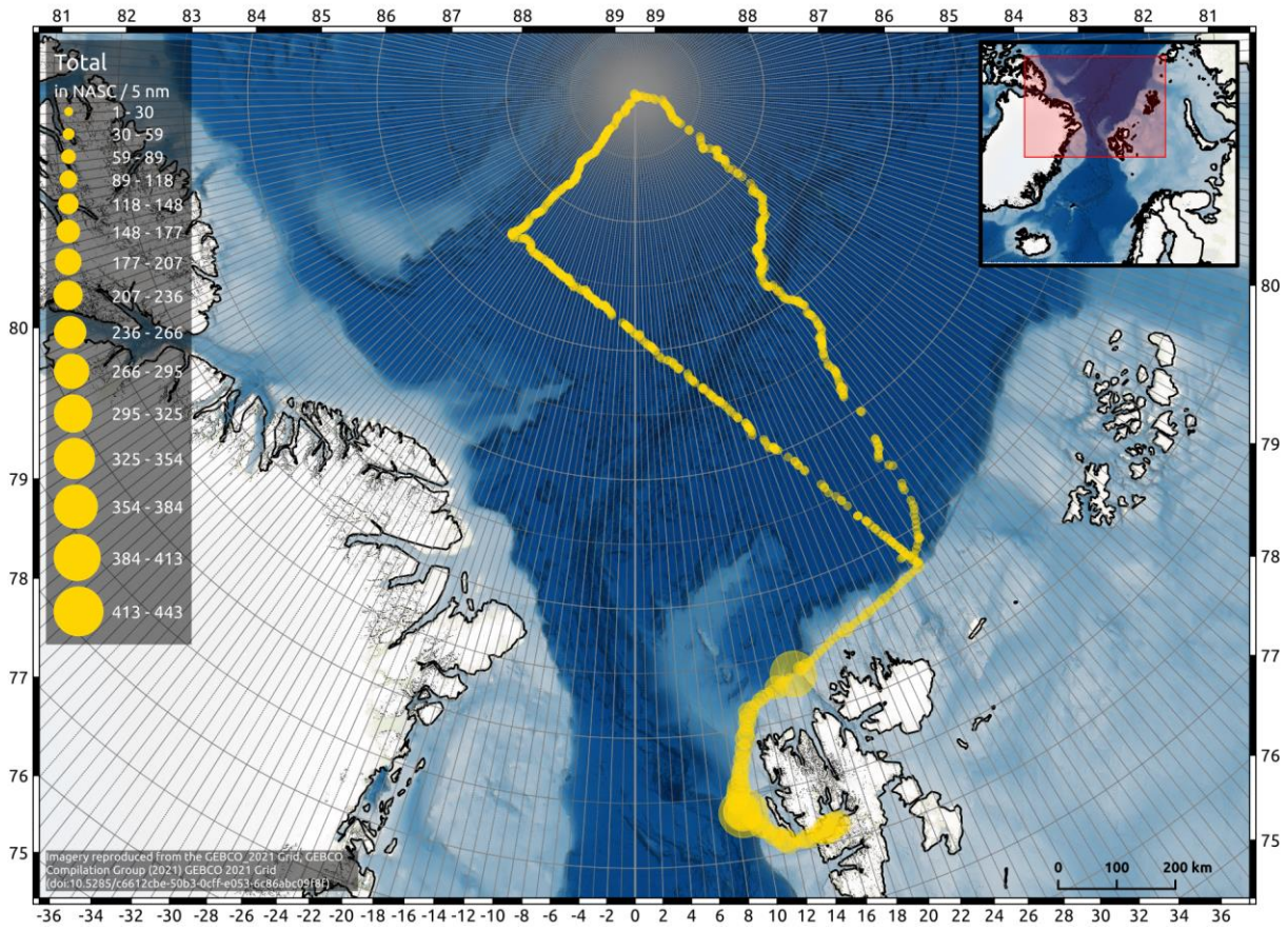
Figure 12. Recordings (Nautical Area Scattering Coefficients/5 nautical mile) made by the Simrad EK80 echo sounder and post processed in LSSS during the Arctic Ocean cruise 2022.
