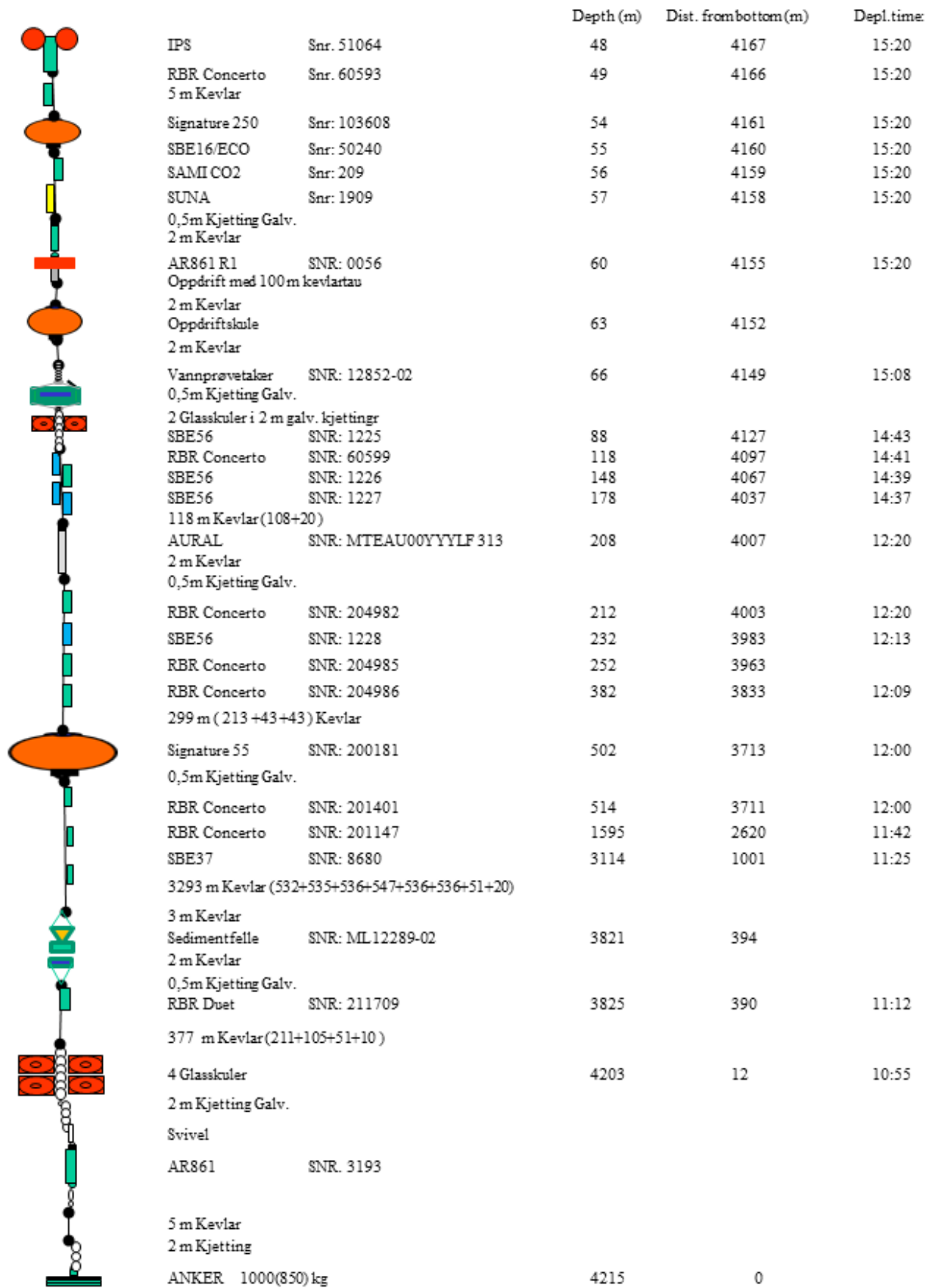
Figure 28. Configuration of the Amundsen-1 mooring.
