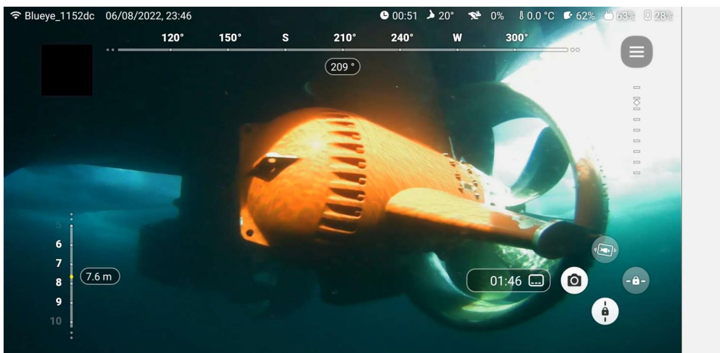
Figure 56. Before retrieving the vehicle, and because navigation with the Hipap system was reliable, the was used to inspect the propellers at the aft of the vessel.
