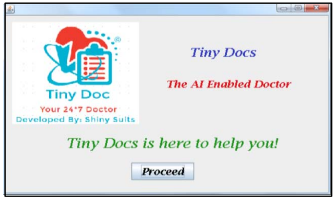
Fig. 7: Gui application
