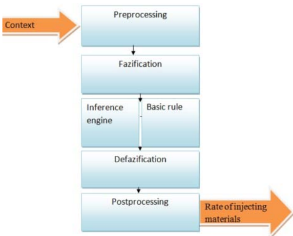
Fig3 : fuzzy controller
