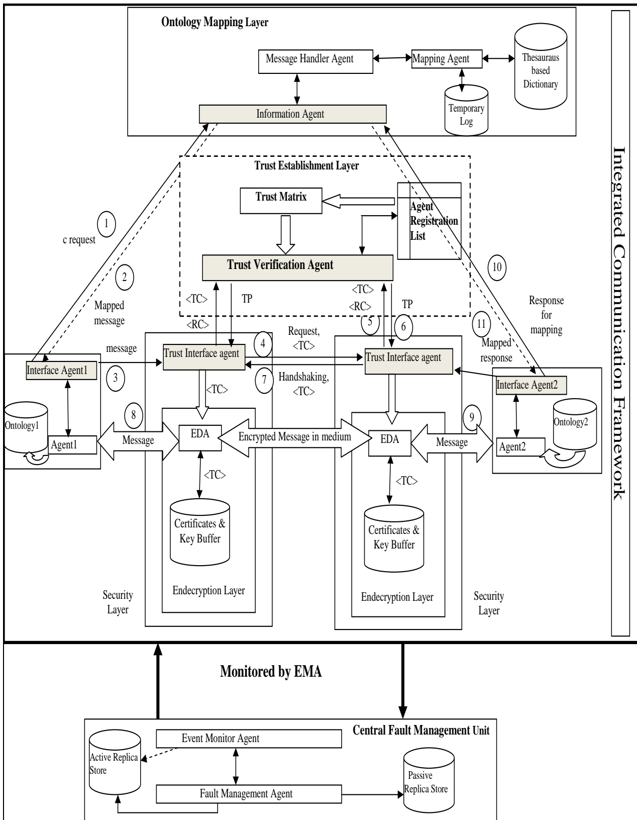
Fig. 1 : High Level View of Multi-Agent Framework for Semantic Web (MAFSW)
