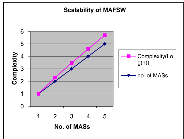
Fig. 4 : Complexity follows Logarithmic Function
