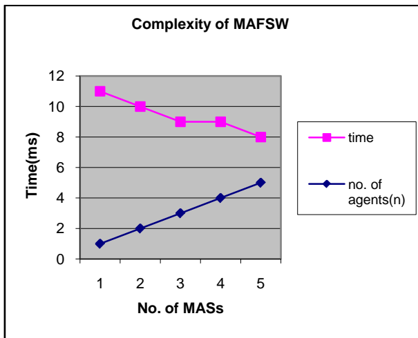
Fig. 3 : Time Reduces with Increase in no. of Participants
