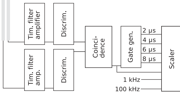
FIG. 3. Schematic of the electronics setup.
