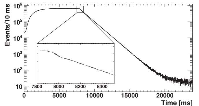
FIG. 4. Histogram for a full {}^6\text{He} counting cycle for the data with initial rates < 40 kHz and the stainless steel insert out. The insert zooms into the transition point from beam on to beam off at which the valve in front of the measuring volume closes and the valve to the roughing pump opens.
