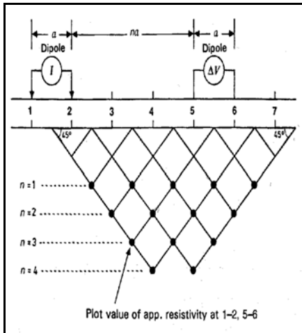
Fig. 1: Scheme of resistivity pseudosection (Dipole-Dipole electrodes configuration).
