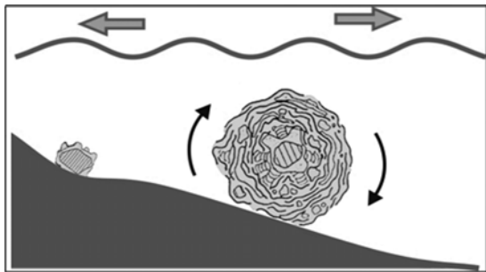
Fig. 14: Formation of coralline algae rhodolithes.
