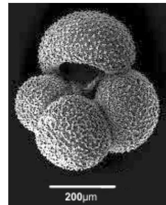
Fig. 16: A Globigerina specimen showing the aggregation of spheroidal chambers.
