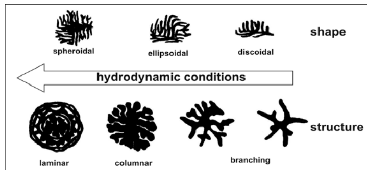
Fig. 15: Relations among rhodolithes shape and structure and hydrodynamic conditions (modified from Bosence, 1991).
