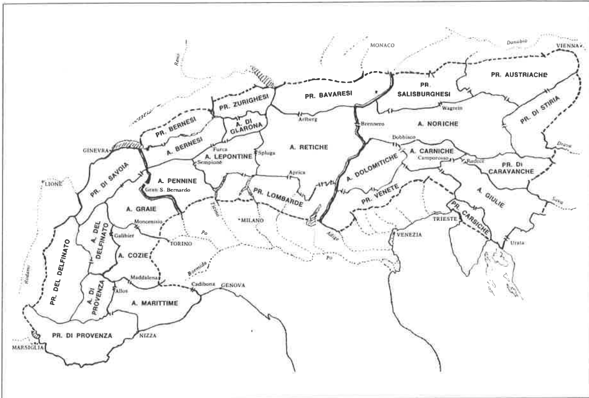
Fig. 1 - The large sectors of the Alpine system (after Bertoglio & De Simoni, 1979).
