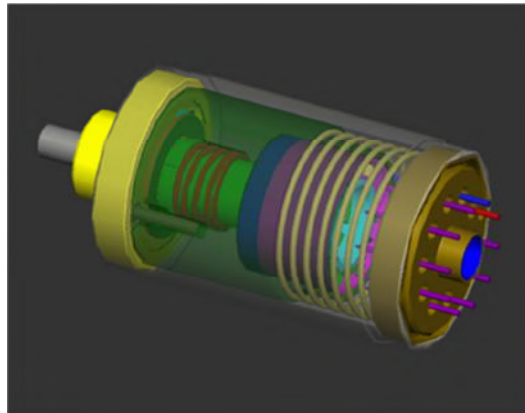
Gambar 2. 1 Accelerometer
