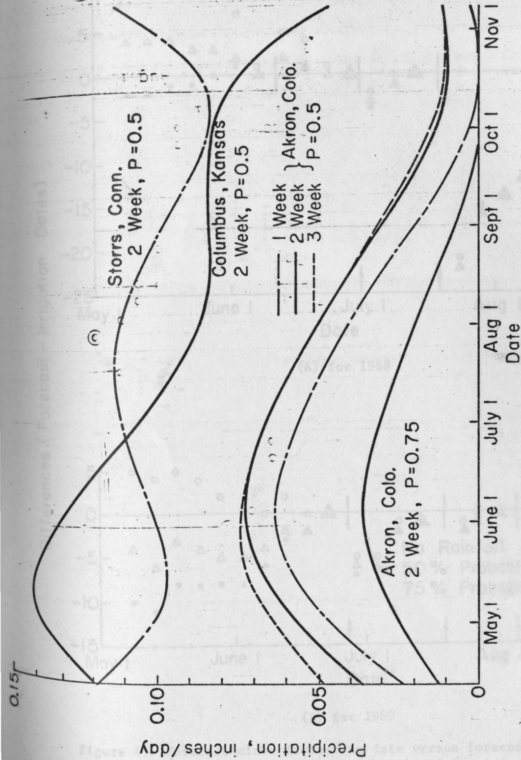
Figure 3. Daily precipitation probabilities from 1-, 2-, 3-week tables for Akron, Colorado, Columbus, Kansas and Storrs, Connecticut.
