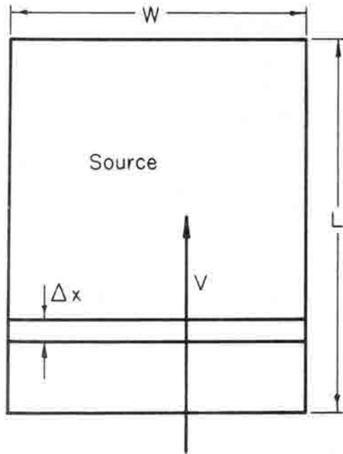
Figure 12. Coordinate system used for calculating models. Symbols are explained in text.
