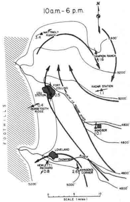
Figure 4a. Resultant streamlines and wind speeds for daytime (10 a.m. - 6 p.m.).
