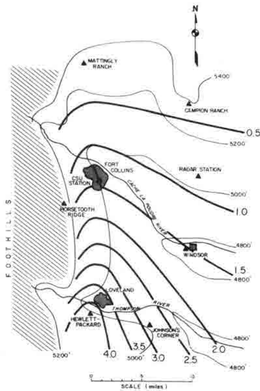
Figure 15d. Same for source of 100 tons/24 hr.
