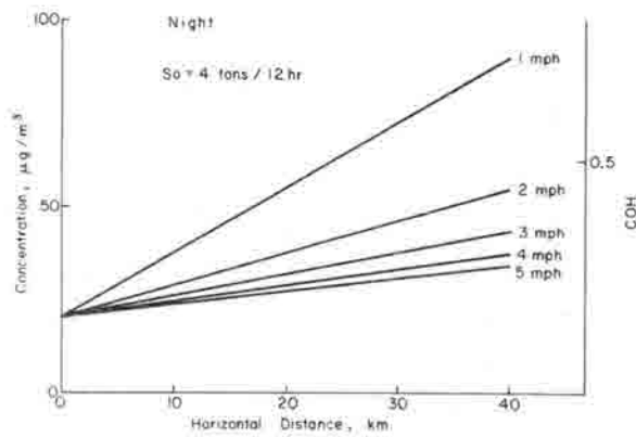
Figure 13. Concentration vs. travel distance for different mean wind speeds for night case with a source of 4 tons/12 hr and initial concentration of 20 \mu\text{g}/\text{m}^3 .
