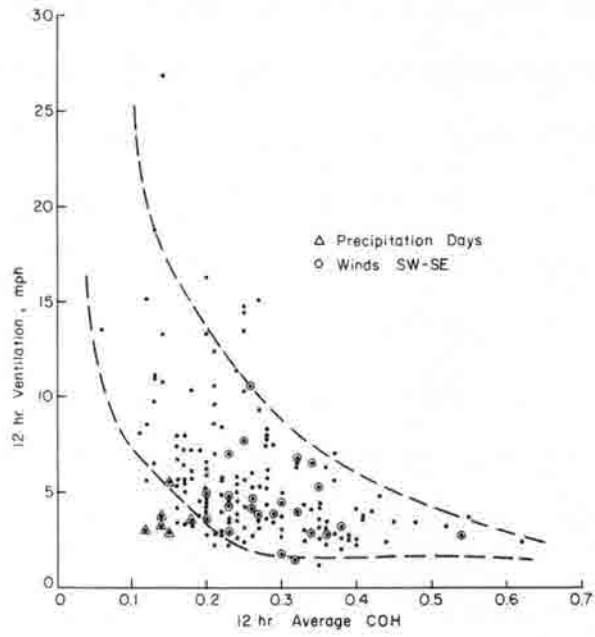
Figure 6. Relation between 12-hr averaged ventilation and COH.
