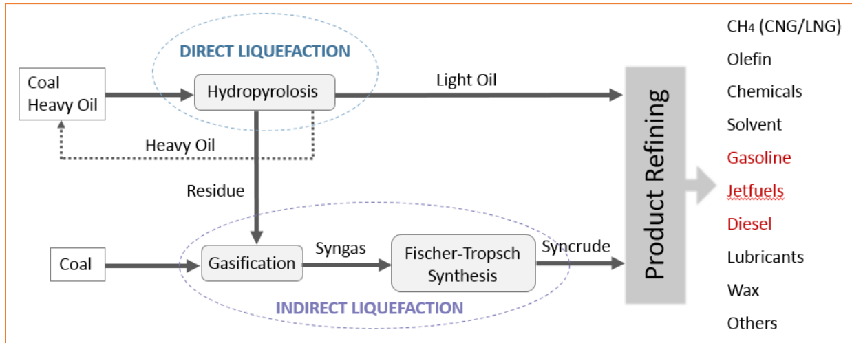
Figure 2D. Simplified Stepwise Liquefaction Process
