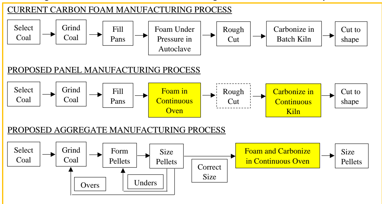
Figure 2E. Carbon Foam Panel Manufacturing Processes Current and Proposed
