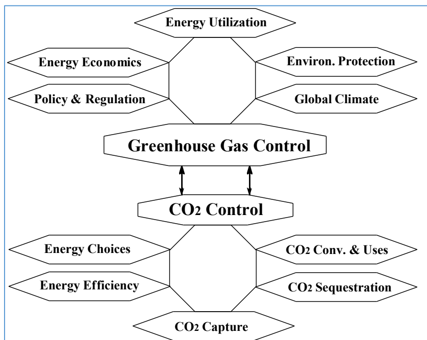
Figure E-15. Key factors in CO 2 control including CO 2 conversion and utilization as chemicals, materials and fuels for CO 2 management
