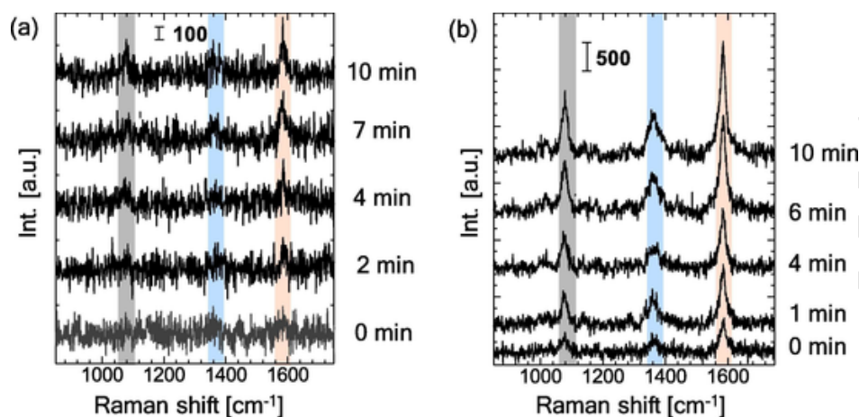
Fig. 8. Raman spectra of PMBA observed under application of an electric field at 50 V/mm at 1 kHz for different application times ranging from 0 to 10 min in the presence of Au@hSiO 2 (a) and m-Au@hSiO 2 (b).
