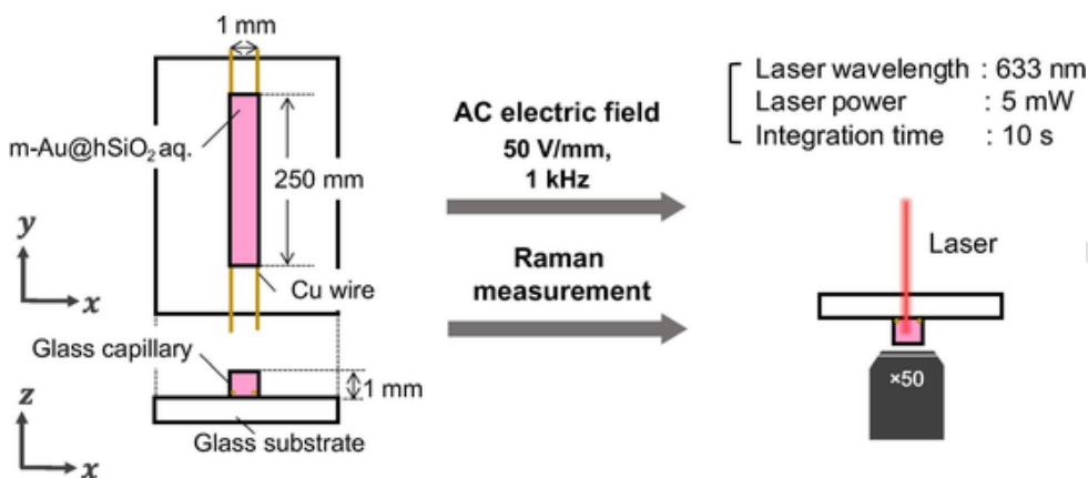
Fig. 2. Schematic procedure of Raman measurement under application of an AC electric field.
