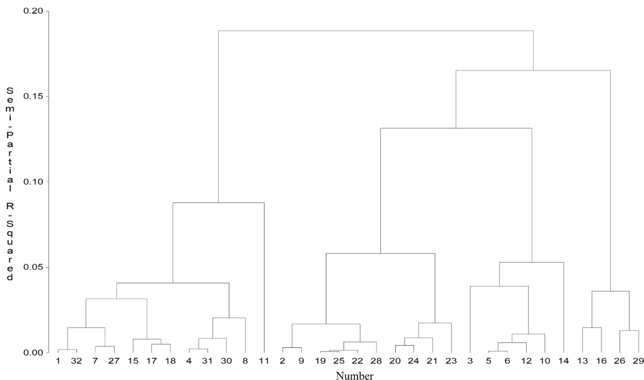
Figure 2. Dendrogram of the rice soils of 32 farms in Majagual, Sucre.
