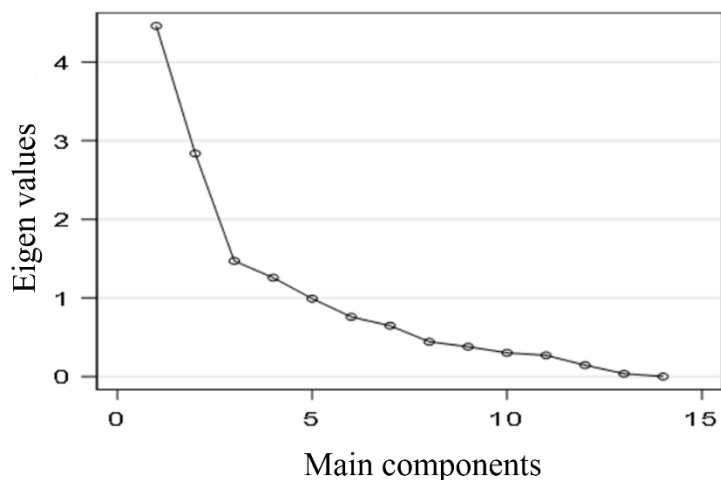
Figure 1. Sedimentation of eigenvalues. Source: Authors
